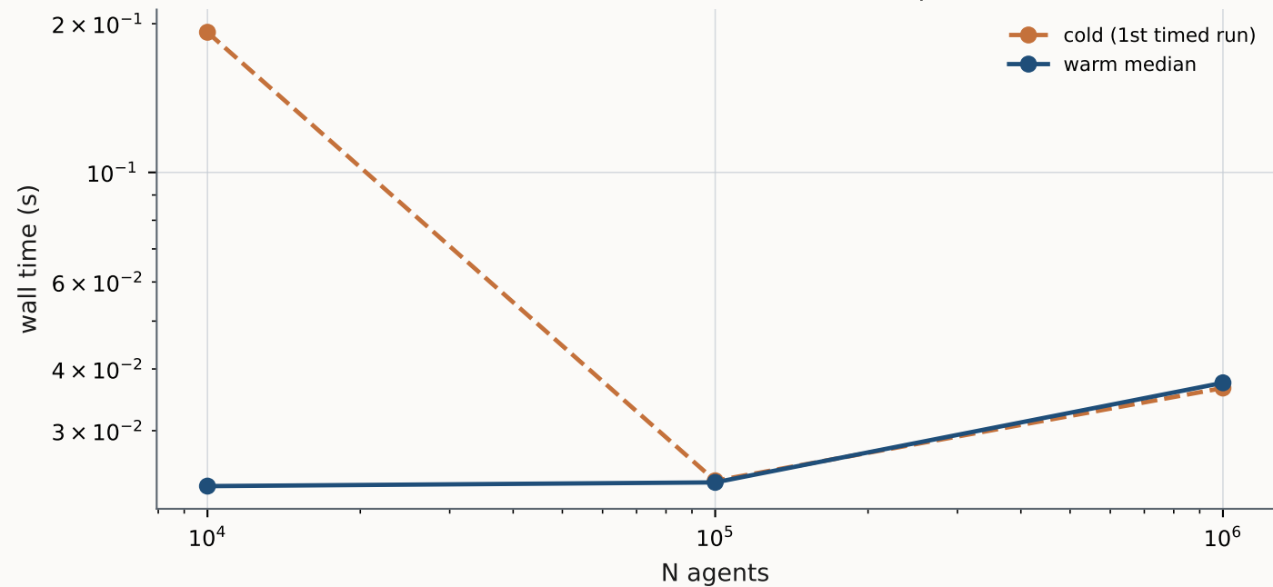
AMBER GPU wealth — cold vs warm separation
