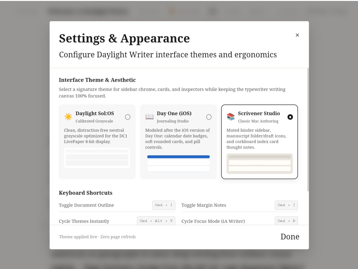
Figure: Surface 6: Settings & Theme Switcher Modal (Interactive Mini-Previews) (File: screenshots/state_12_settings_theme_modal_hardware.png)
