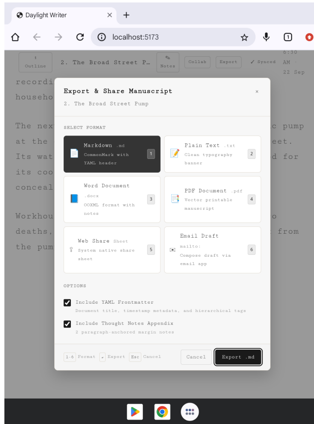
Figure: Surface 8: Multi-Format Export Dialog (.md, .txt, .docx, .pdf, Android SAF) (File: screenshots/state_6_export_dialog_hardware.png)
