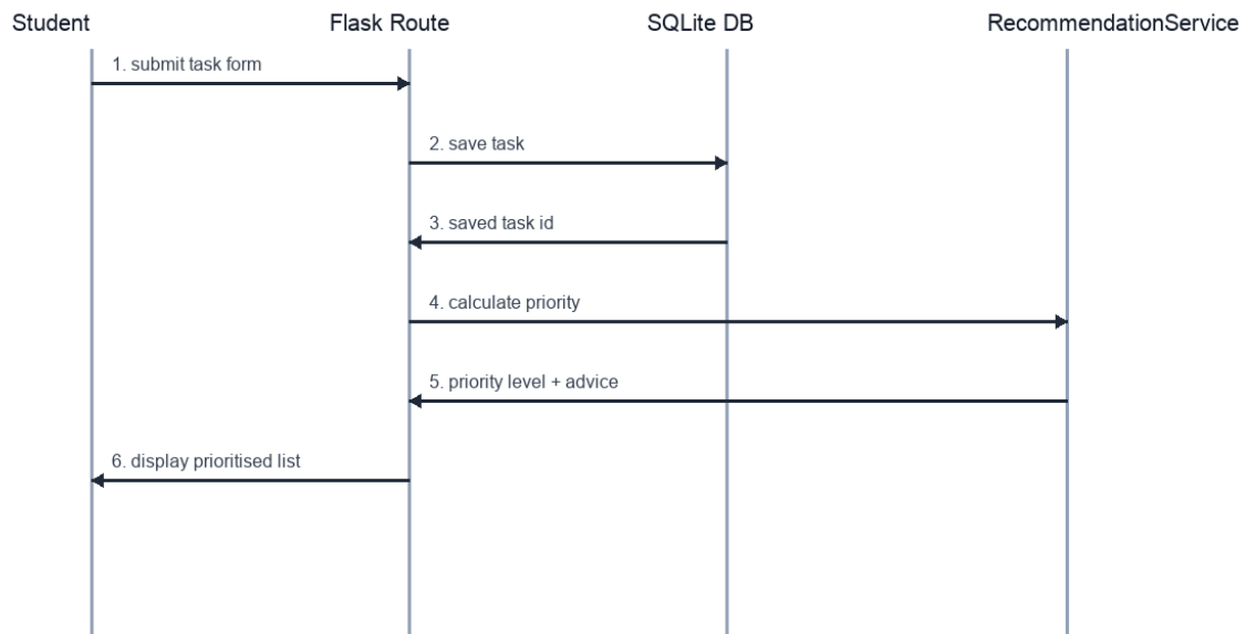
Sequence Diagram - Add Task and Generate Priority
