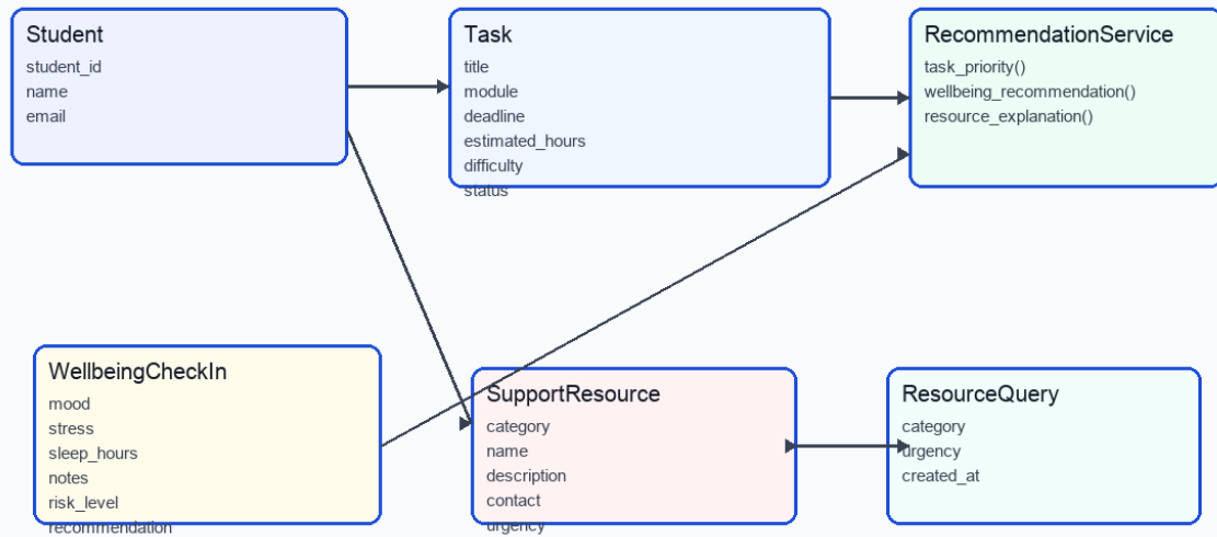
Class Diagram - UniHelp Planner
