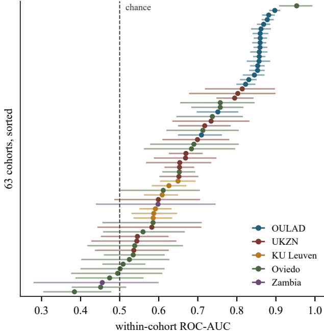
Fig. 1. Within-cohort ROC-AUC for every cohort, sorted, with 400-resample bootstrap intervals over students; colour marks the institution. Institution accounts for 57.3% of the variance, but not cleanly: cohort size correlates 0.669 with AUC and is itself collinear with institution.
