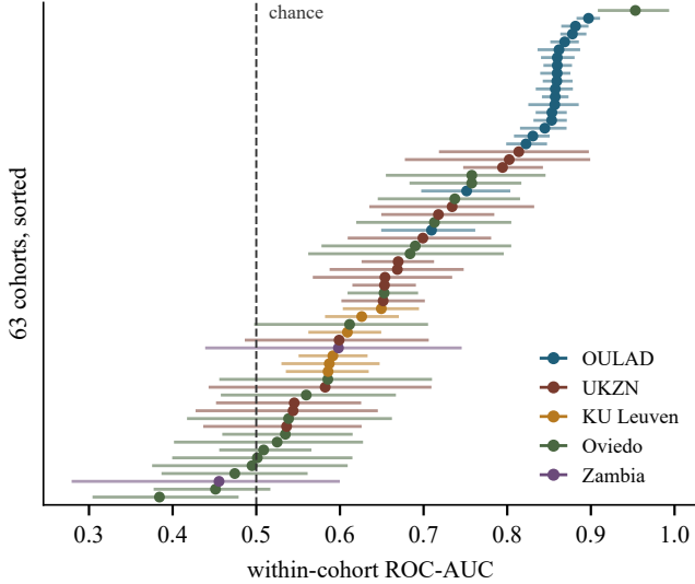
Fig. 1. Within-cohort ROC-AUC for every cohort, sorted, with 400-resample bootstrap intervals over students; colour marks the institution. Institution accounts for 57.3 % of the variance, but not cleanly: cohort size correlates 0.669 with AUC and is itself collinear with institution.
