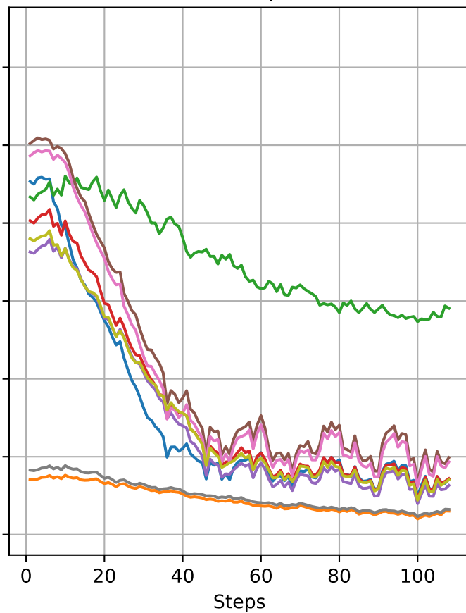
LifeSnaps
