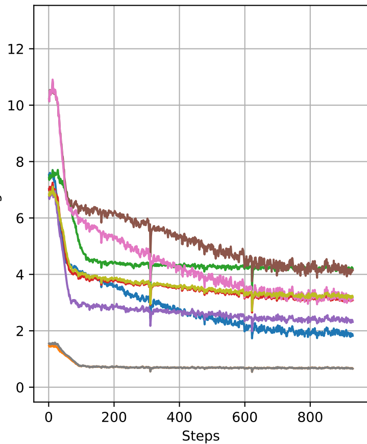
PMData
