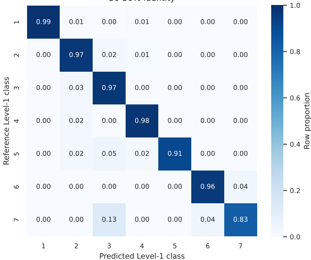
30-50% identity
