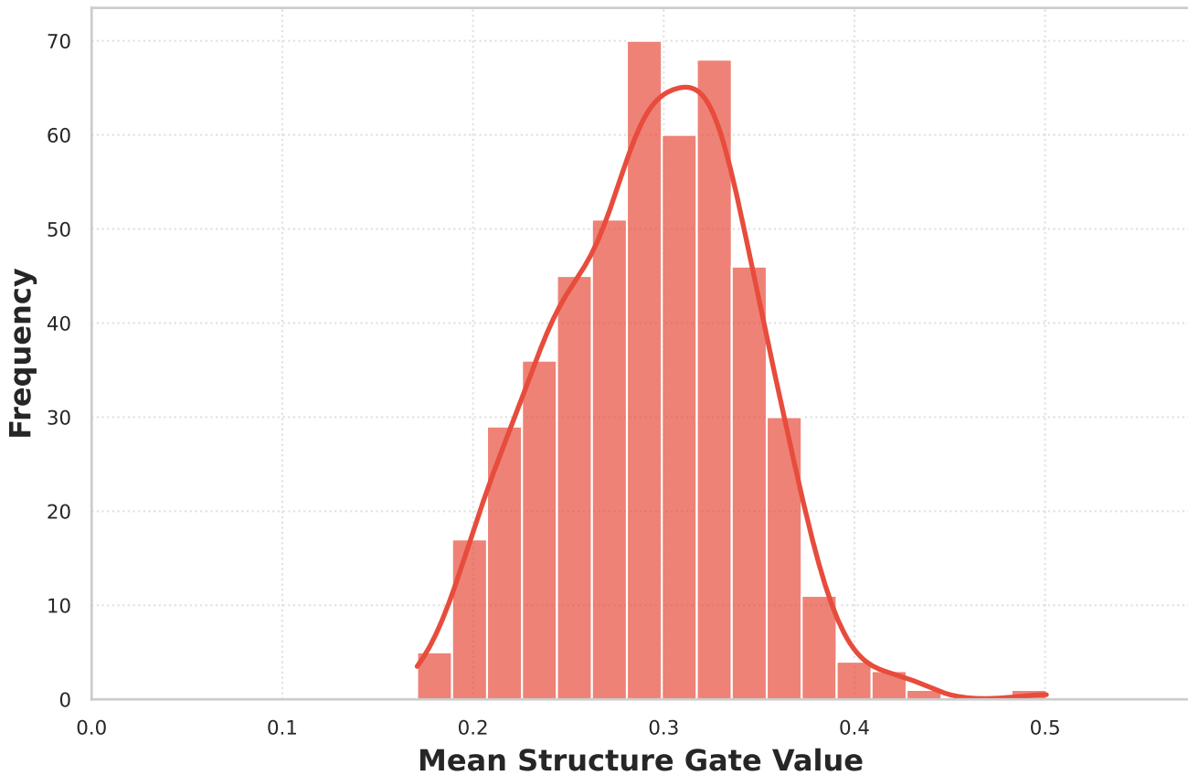
Distribution of Gating Weights (30-50%)
