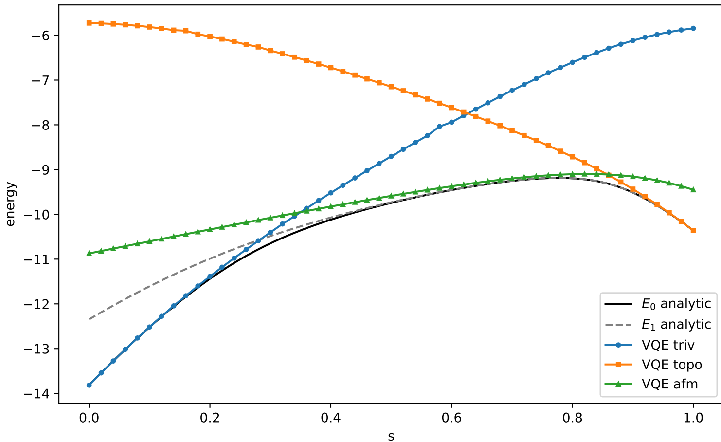
VQE vs analytic, H (L=8, delta=+1)
