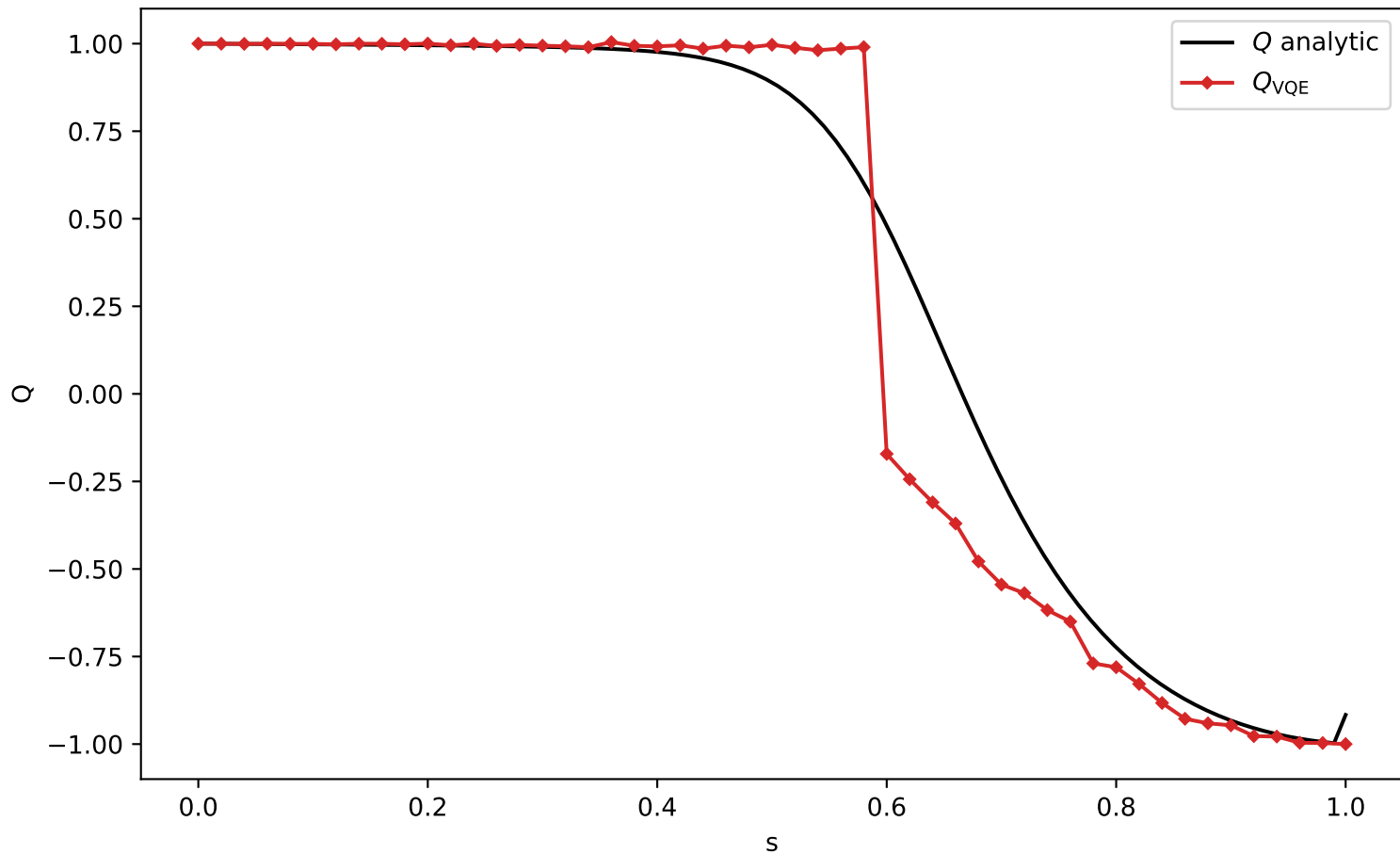
Q-orbit vs analytic (L=8, depth=1, delta=-1)
