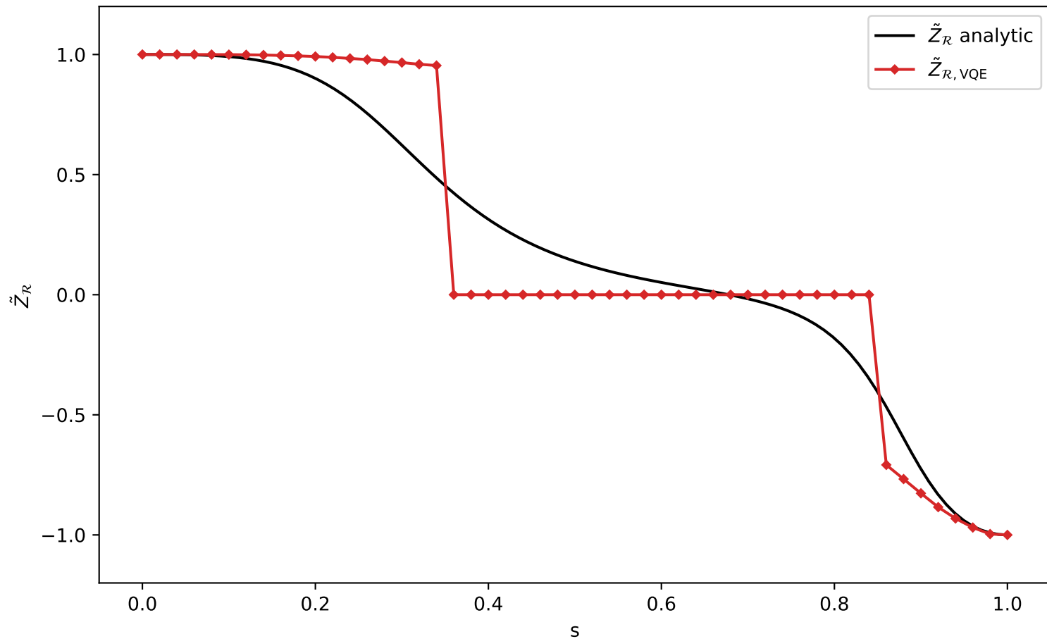
ZR-orbit vs analytic (L=8, depth=1, delta=1)
