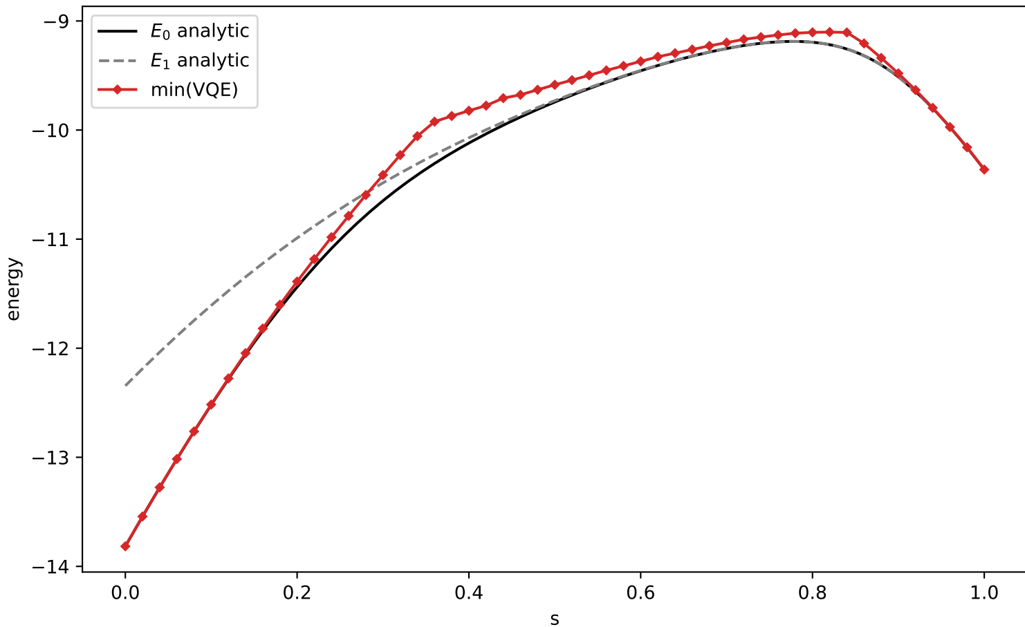
VQE-orbit vs analytic (L=8, depth=1, delta=1)
