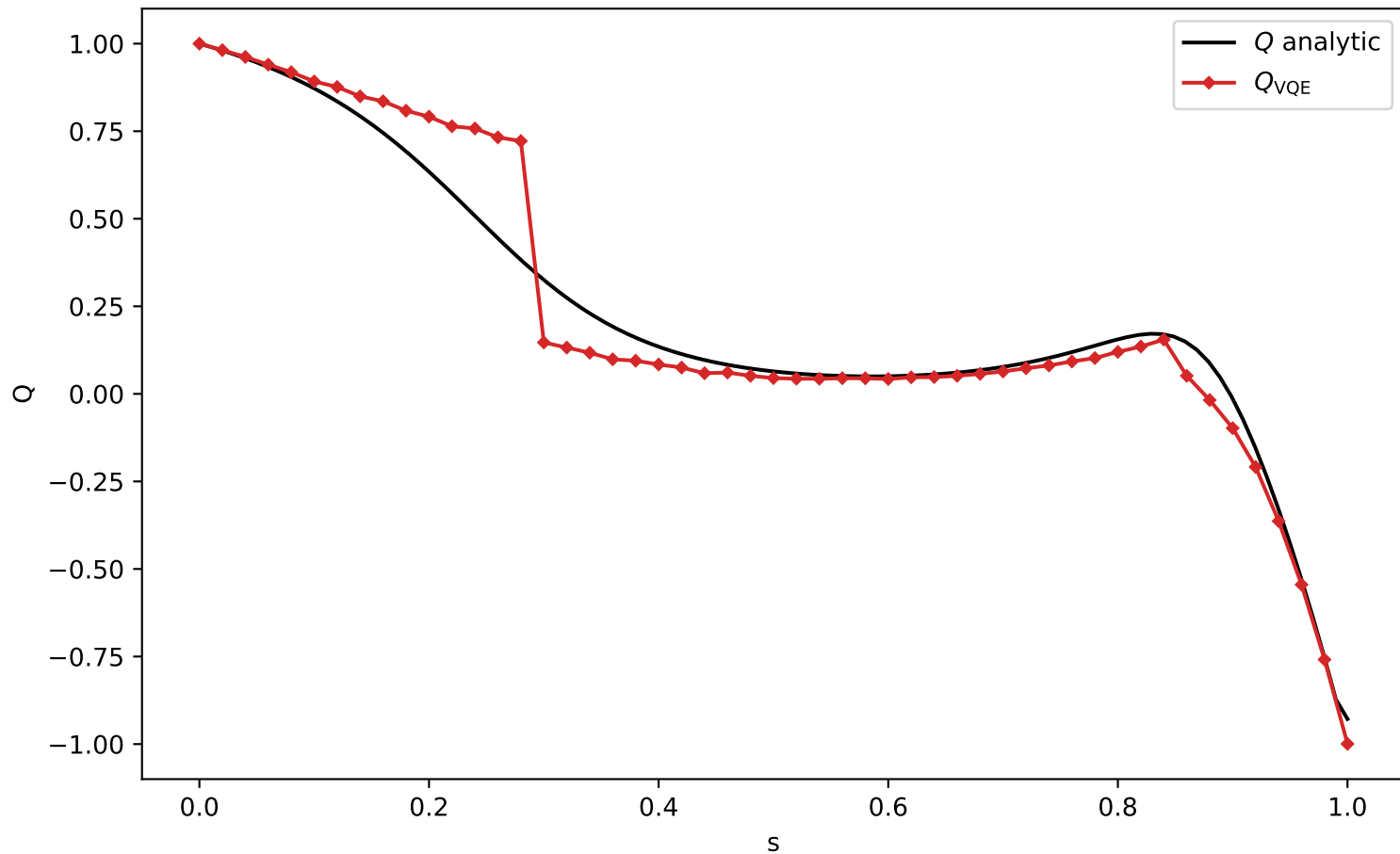
Q-orbit vs analytic (L=8, depth=2, delta=1)
