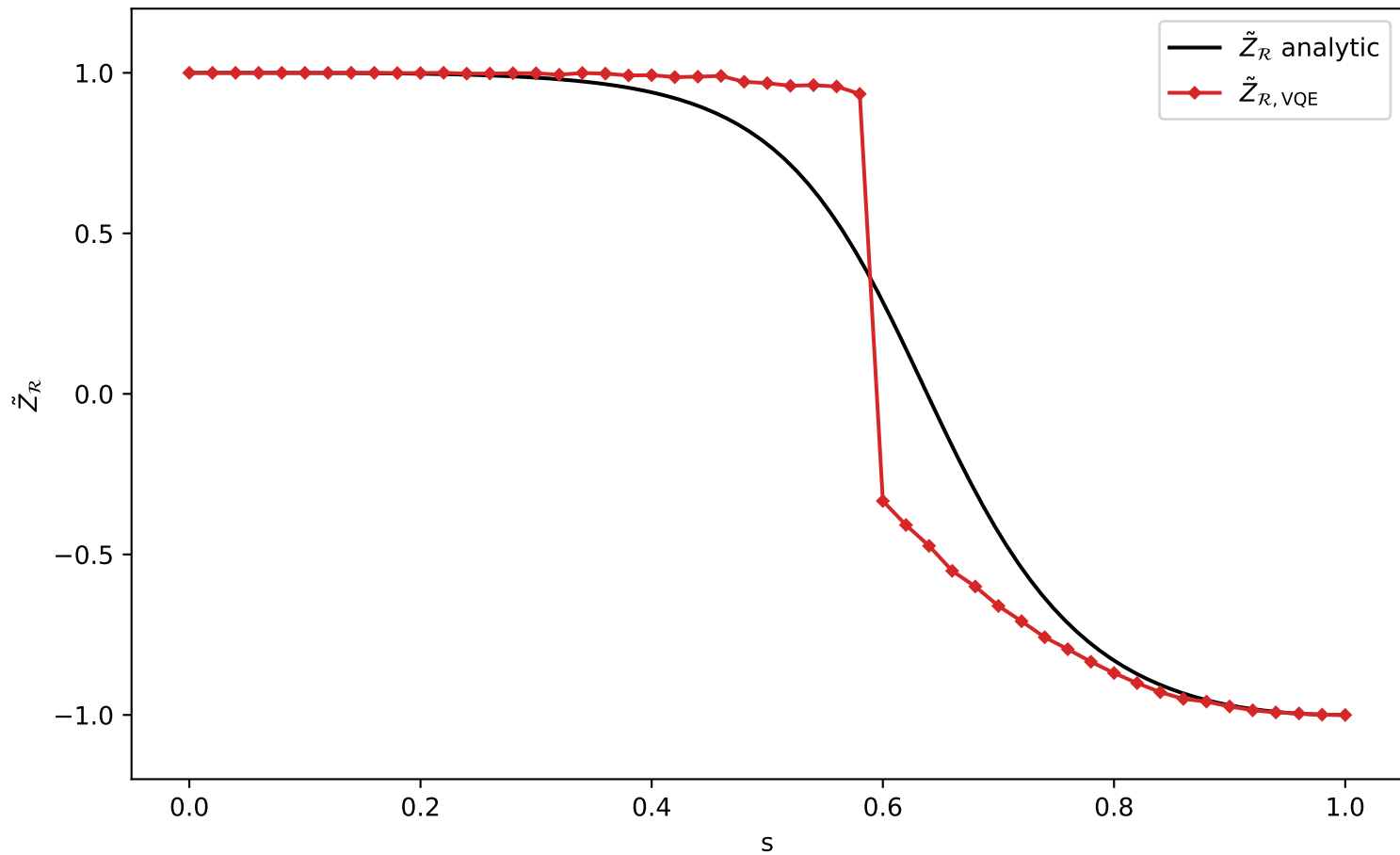
ZR-orbit vs analytic (L=8, depth=2, delta=-1)
