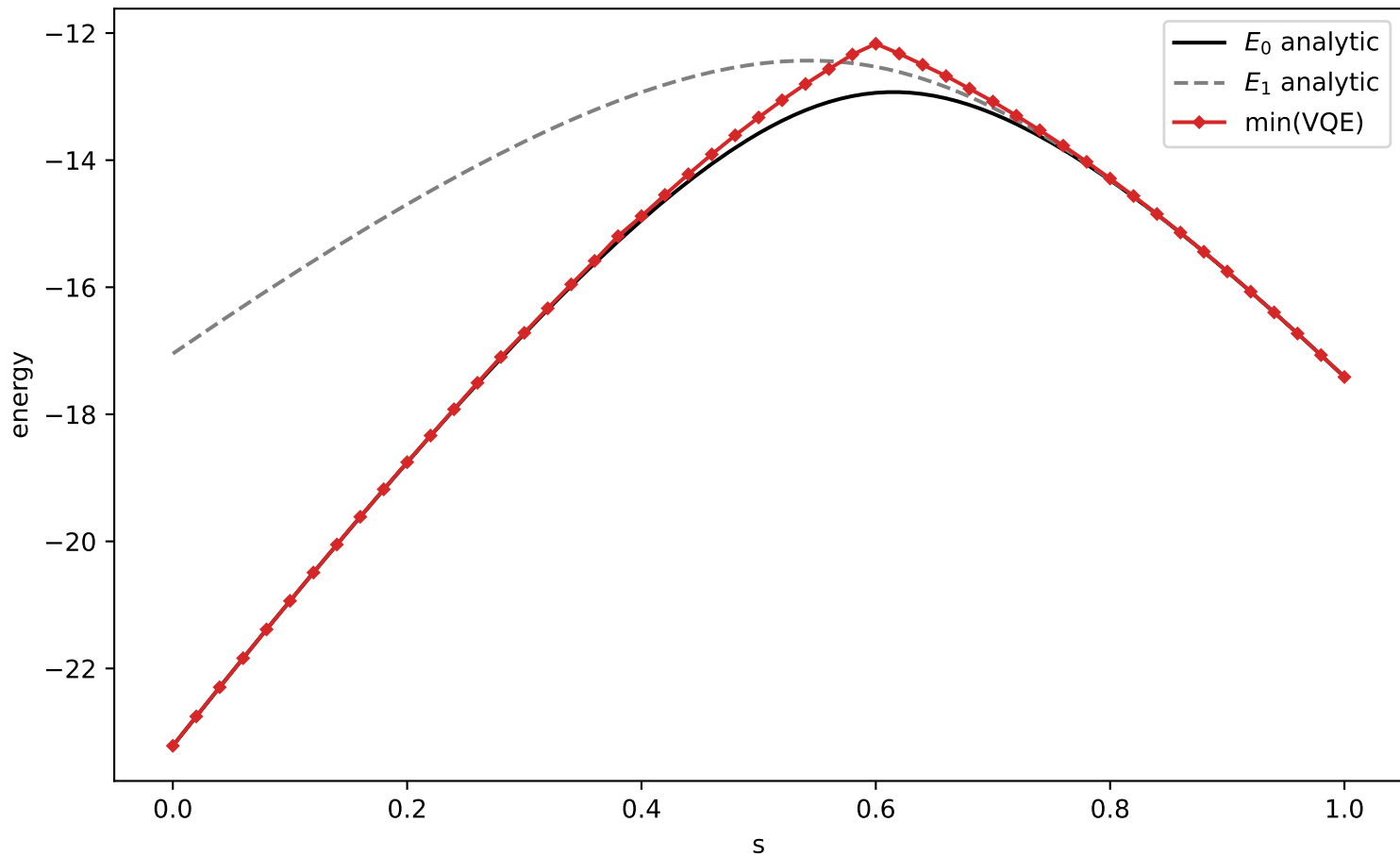
VQE-orbit vs analytic (L=8, depth=2, delta=-1)
