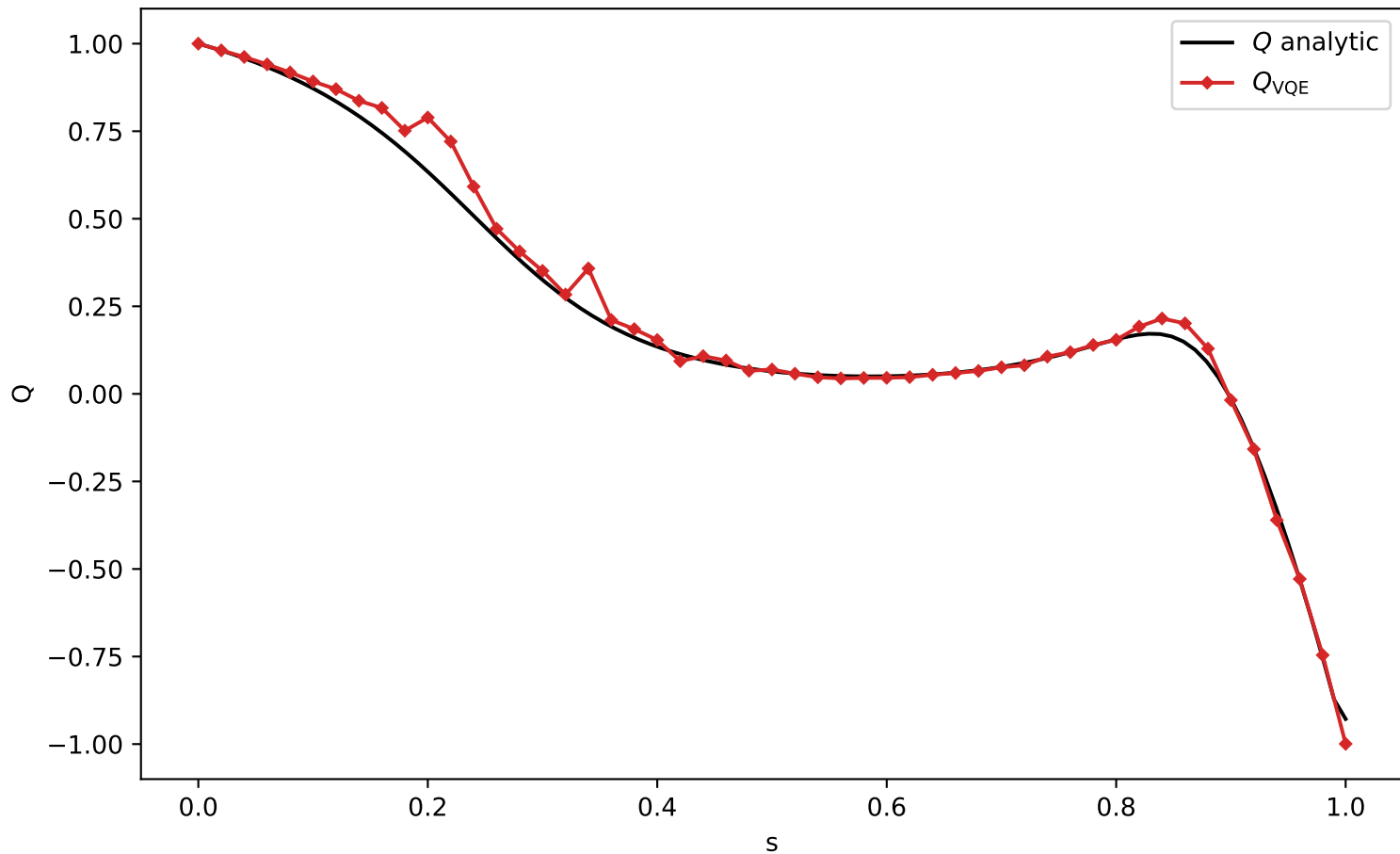
Q-orbit vs analytic (L=8, depth=3, delta=1)
