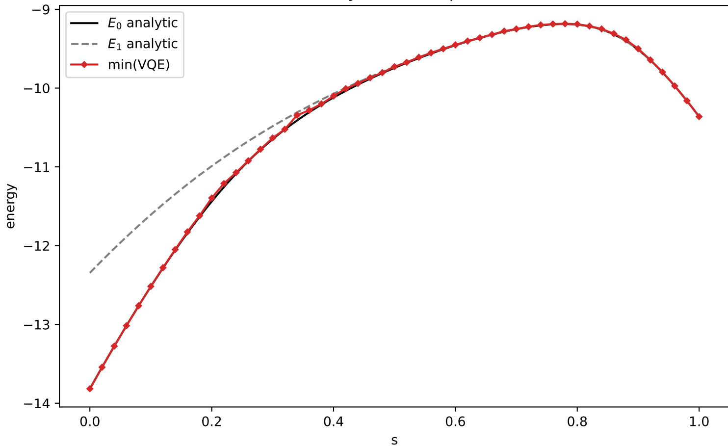
VQE-orbit vs analytic (L=8, depth=3, delta=1)
