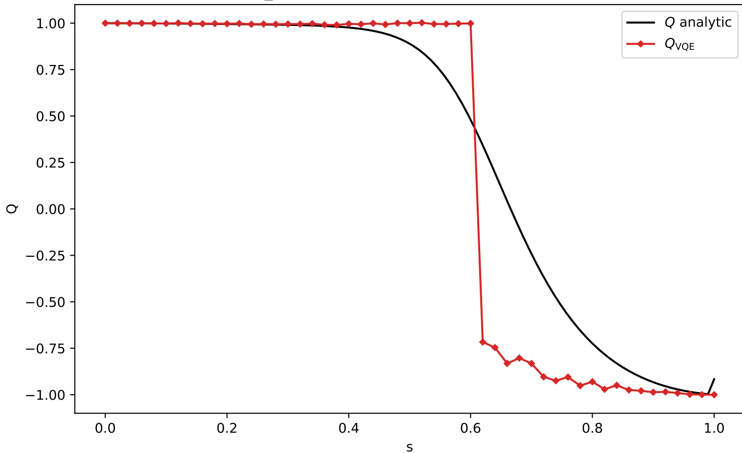
Q_VQE vs analytic Q, H (L=8, delta=-1)
