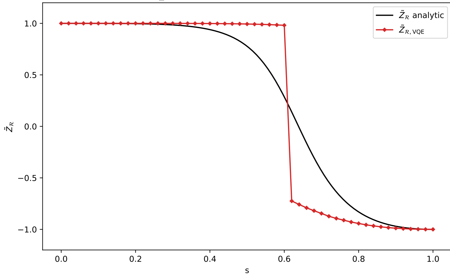
ZR_VQE vs analytic ZR, H (L=8, delta=-1)
