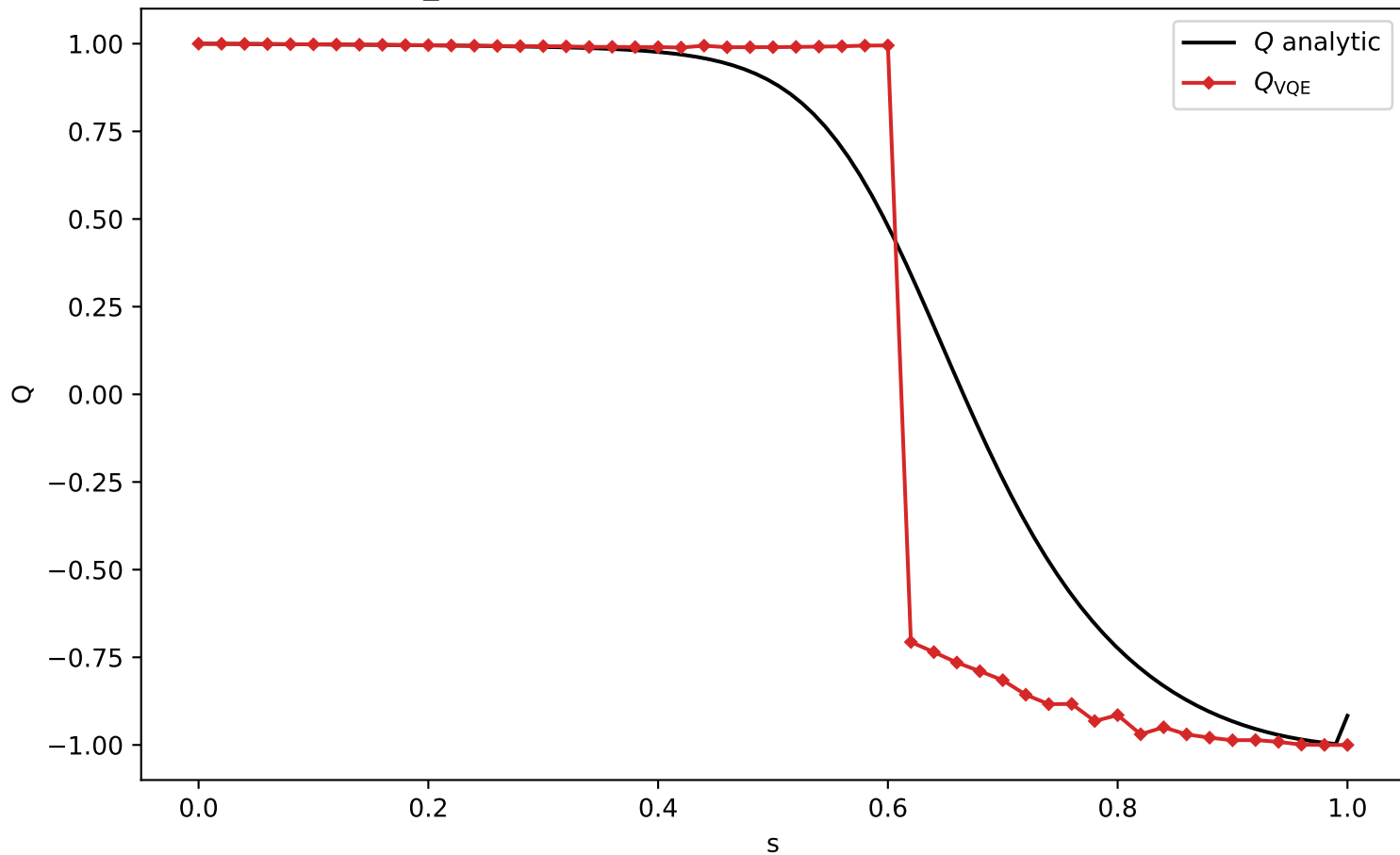
Q_VQE vs analytic Q, H (L=8, depth=2, delta=-1)
