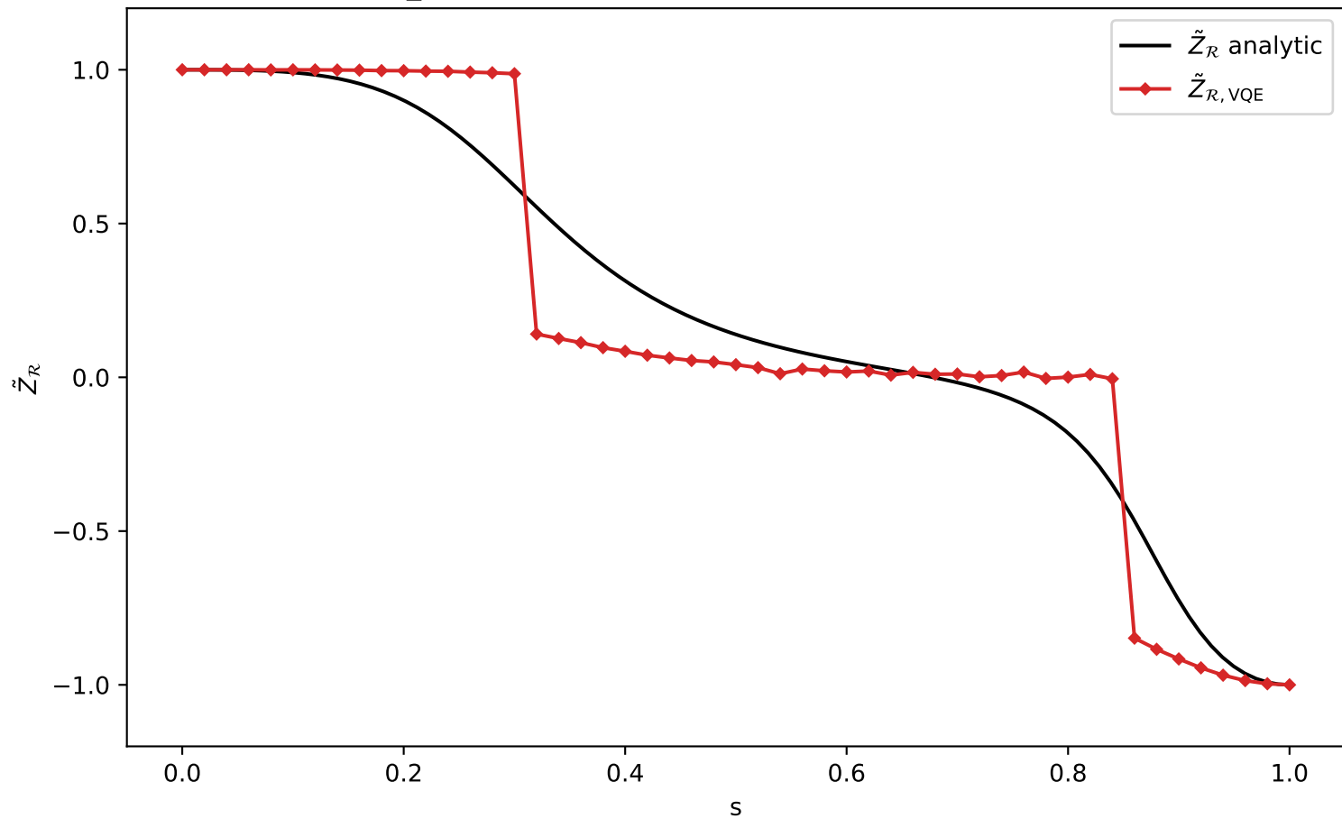
ZR_VQE vs analytic ZR, H (L=8, depth=2, delta=1)
