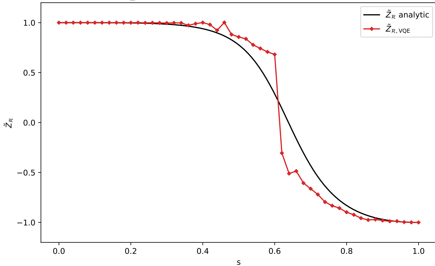
ZR_VQE vs analytic ZR, H (L=8, depth=4, delta=-1)
