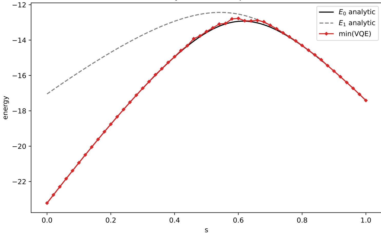
min(VQE) vs analytic, H (L=8, depth=5, delta=-1)
