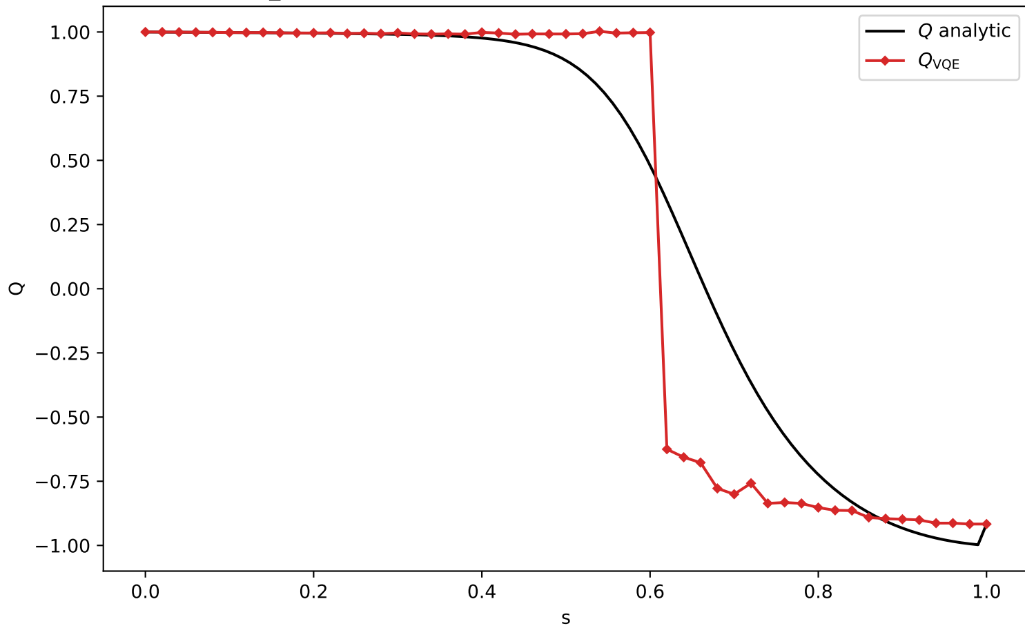
Q_VQE-nosym vs analytic Q, H (L=8, depth=1, delta=-1)
