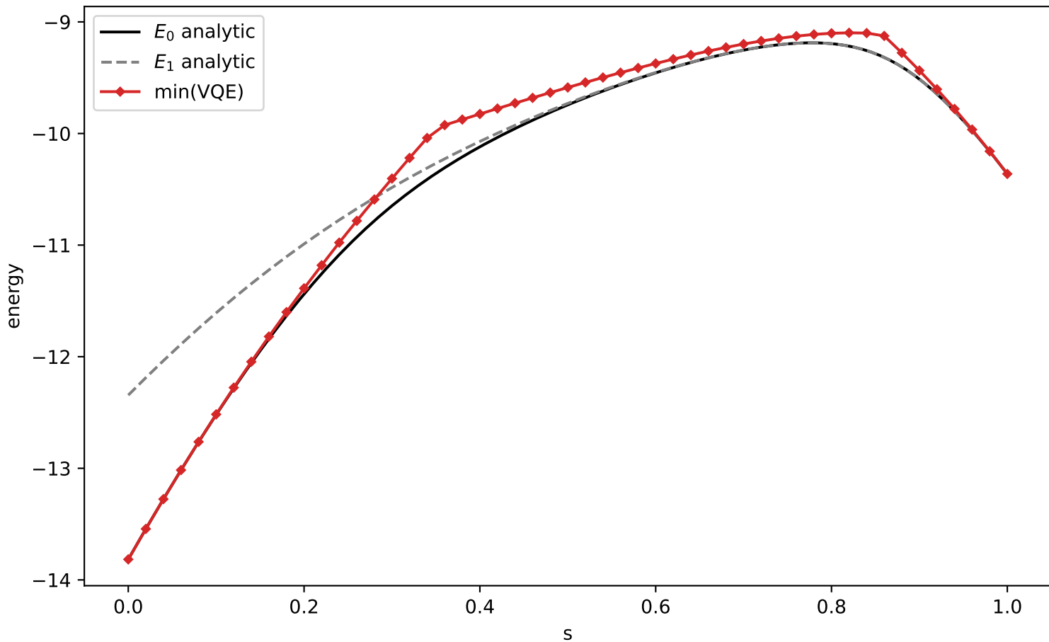
min(VQE-nosym) vs analytic, H (L=8, depth=1, delta=1)
