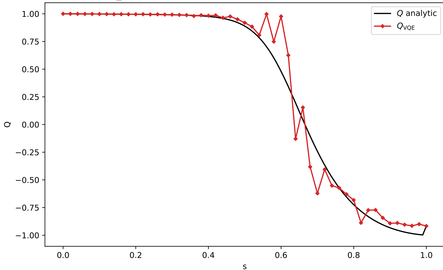
Q_VQE-nosym vs analytic Q, H (L=8, depth=5, delta=-1)
