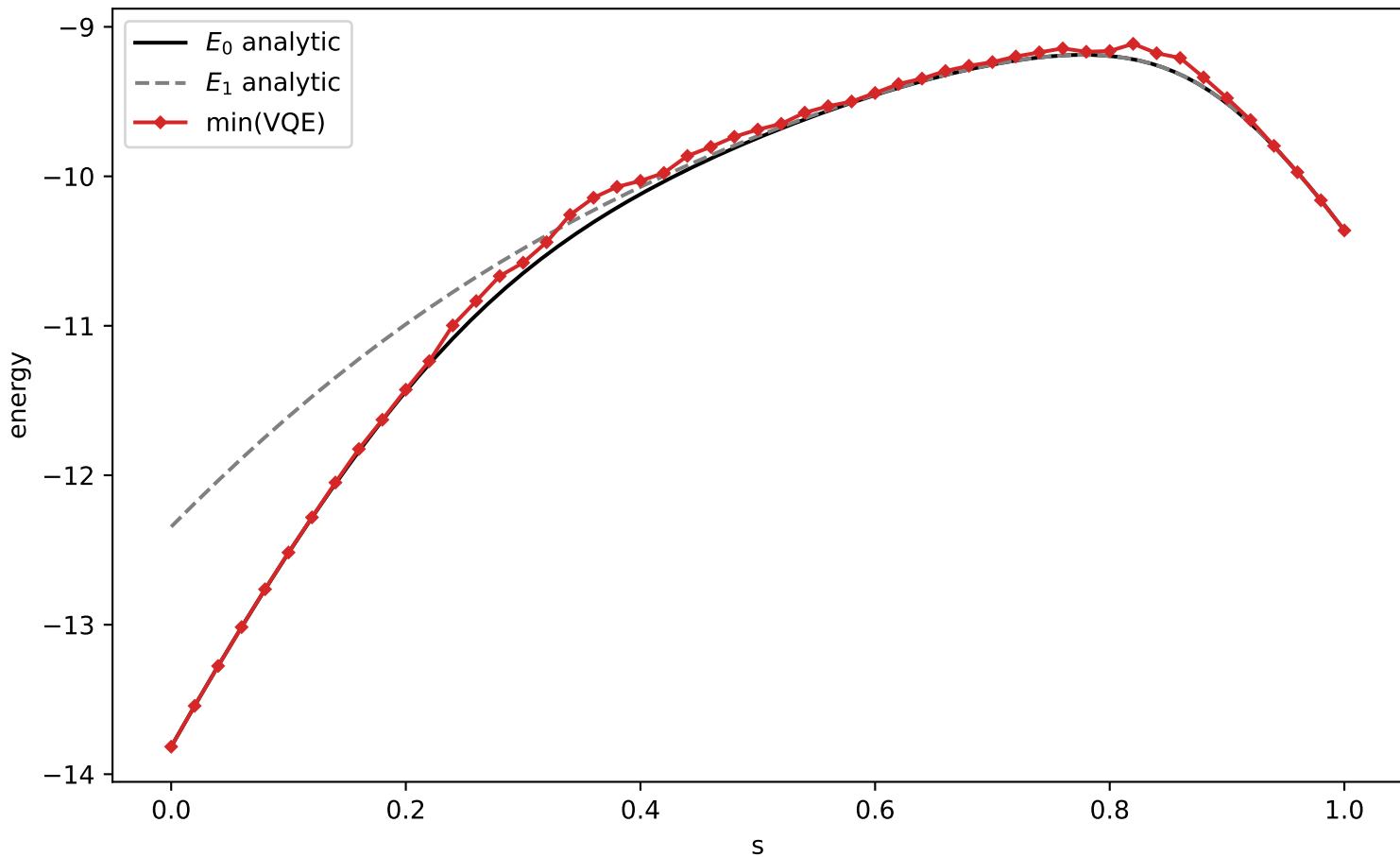
min(VQE-nosym) vs analytic, H (L=8, depth=5, delta=1)
