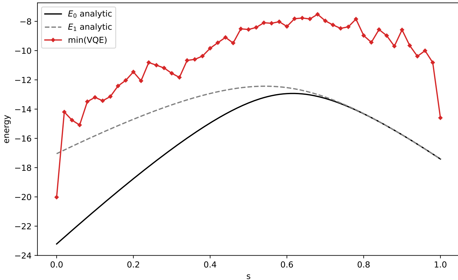
VQE hw nosym depth1 delta=-1.0 min-energy
