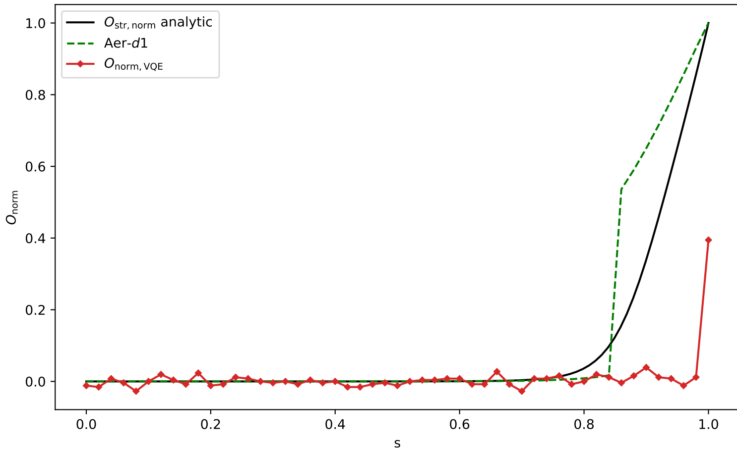
VQE hw+aer nosym depth1 delta=1.0 o
