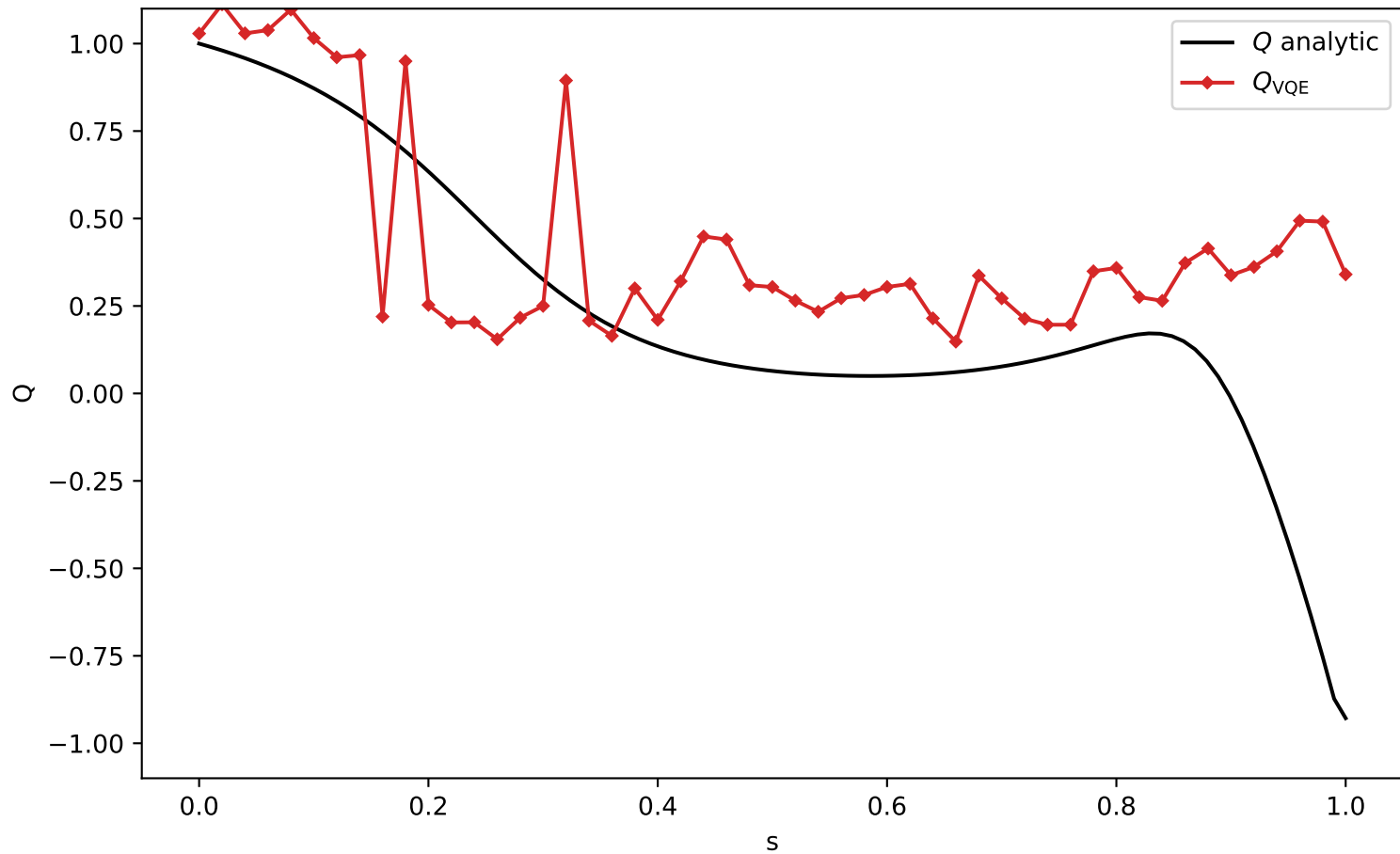
VQE hw nosym depth1 delta=1.0 Q
