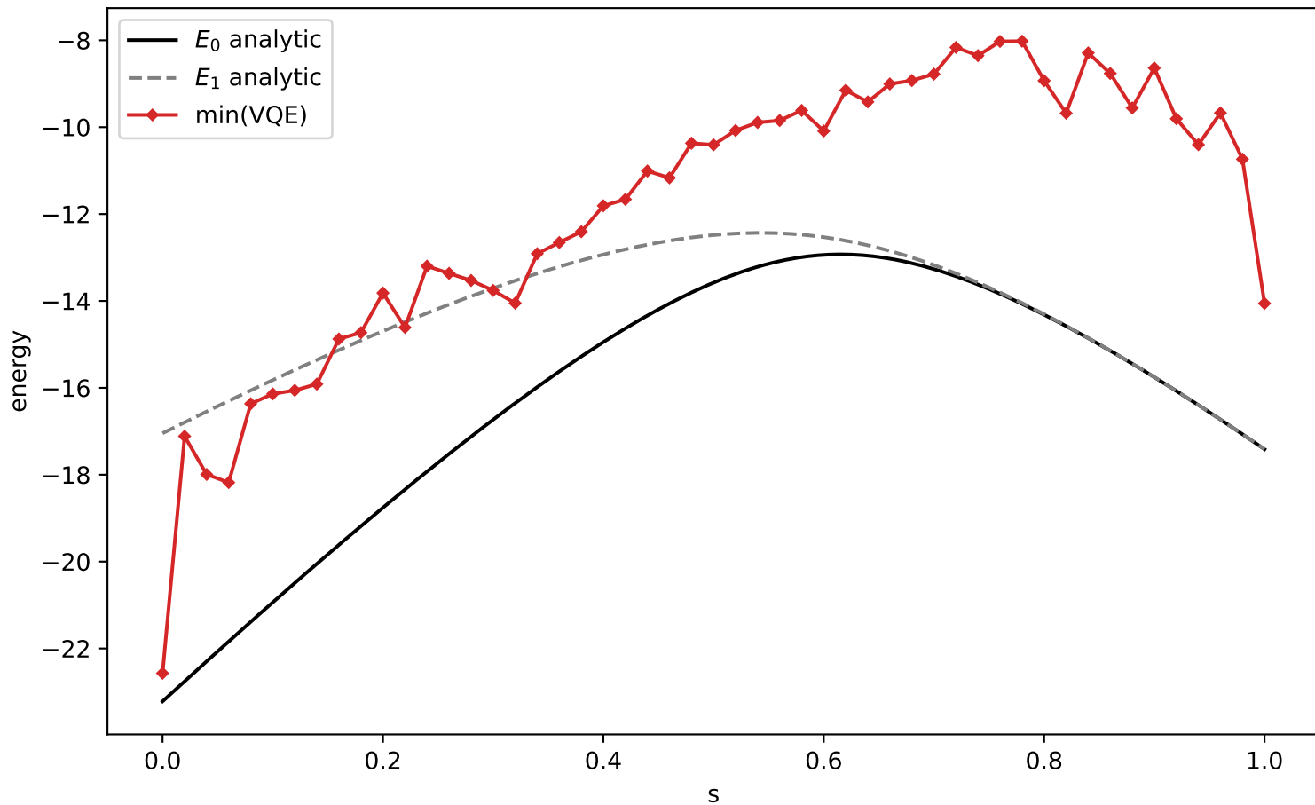
VQE postselect nosym depth1 delta=-1.0 min-Hpost (diagnostic)
