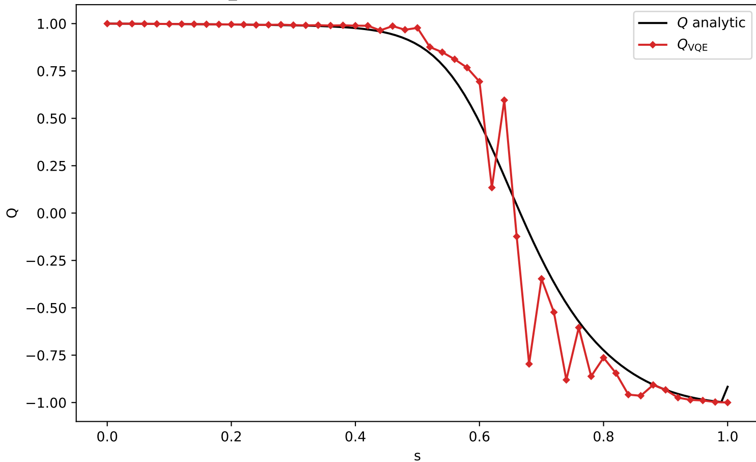
Q_VQE vs analytic Q, H (L=8, depth=3, delta=-1)
