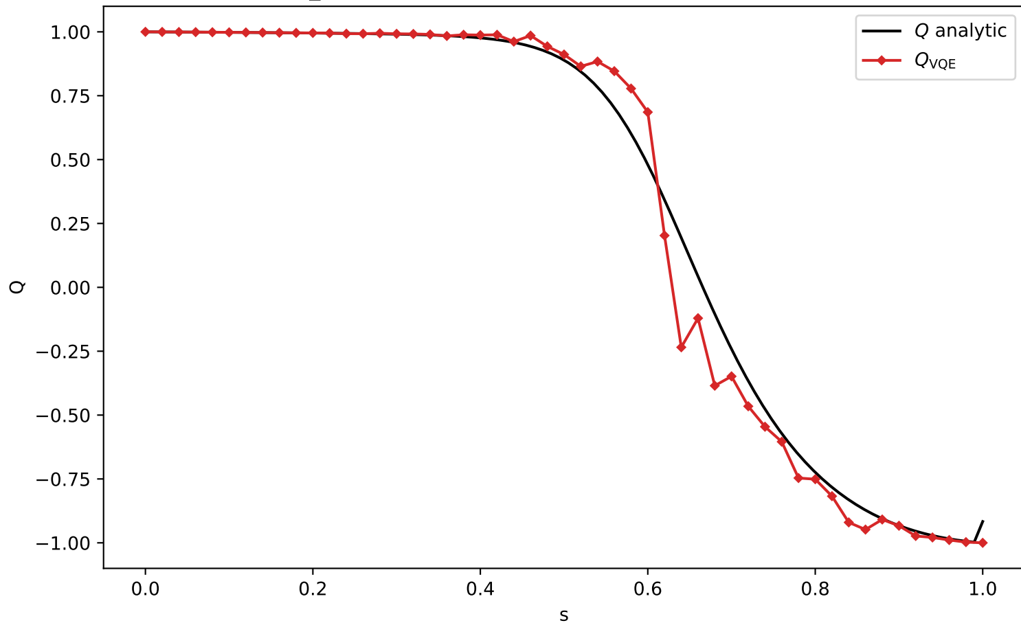
Q_VQE vs analytic Q, H (L=8, depth=4, delta=-1)
