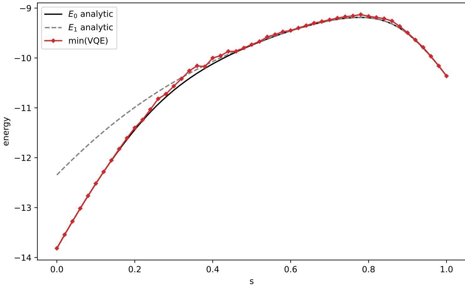
min(VQE) vs analytic, H (L=8, depth=4, delta=1)
