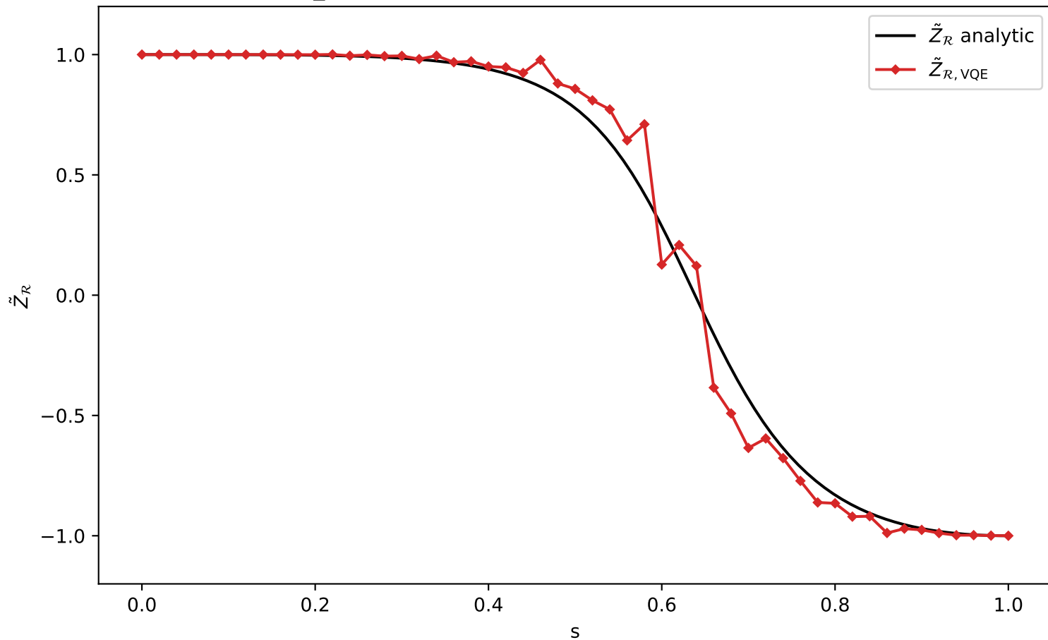
ZR_VQE vs analytic ZR, H (L=8, depth=5, delta=-1)
