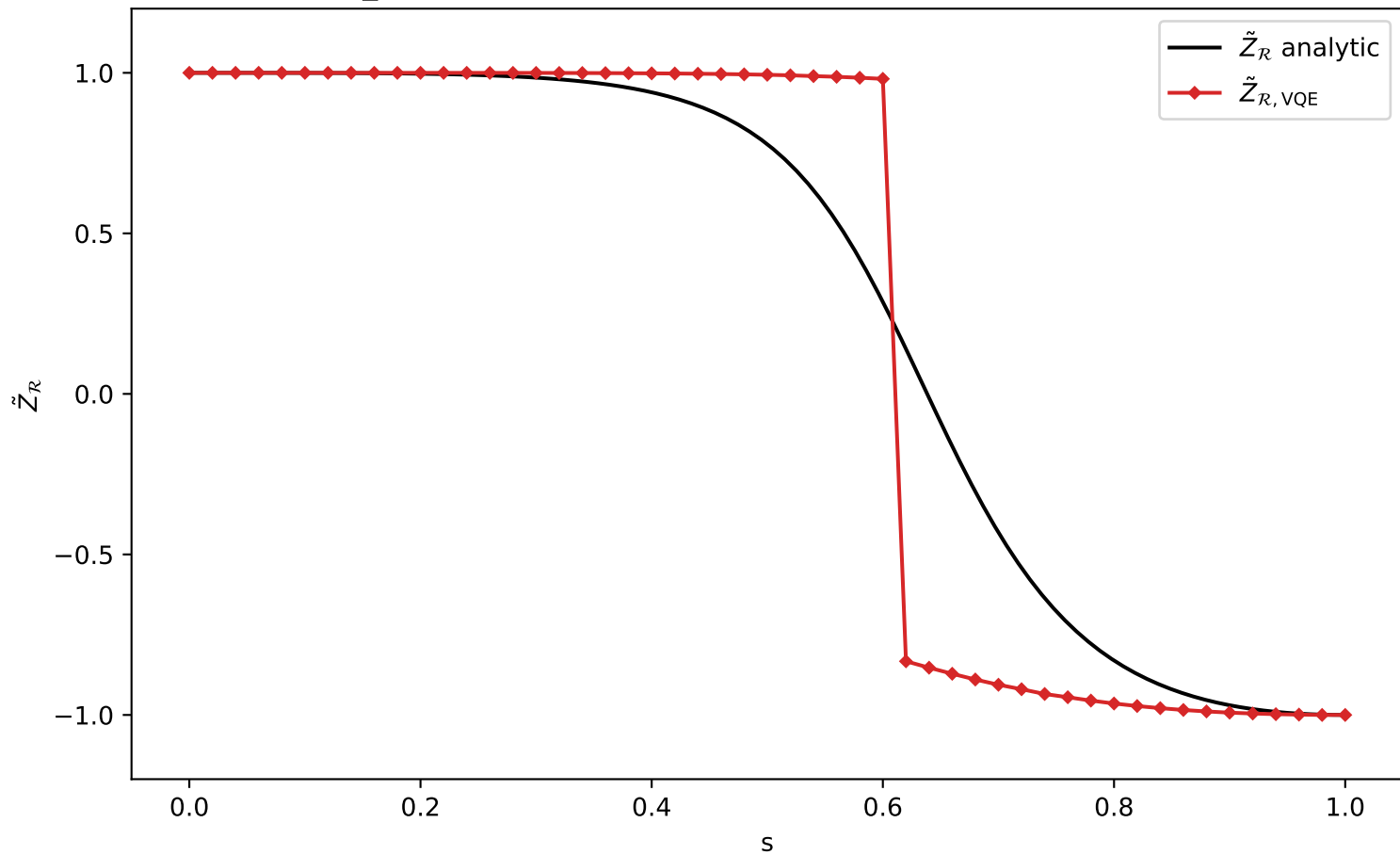
ZR_VQE-nosym vs analytic ZR, H (L=8, depth=1, delta=-1)
