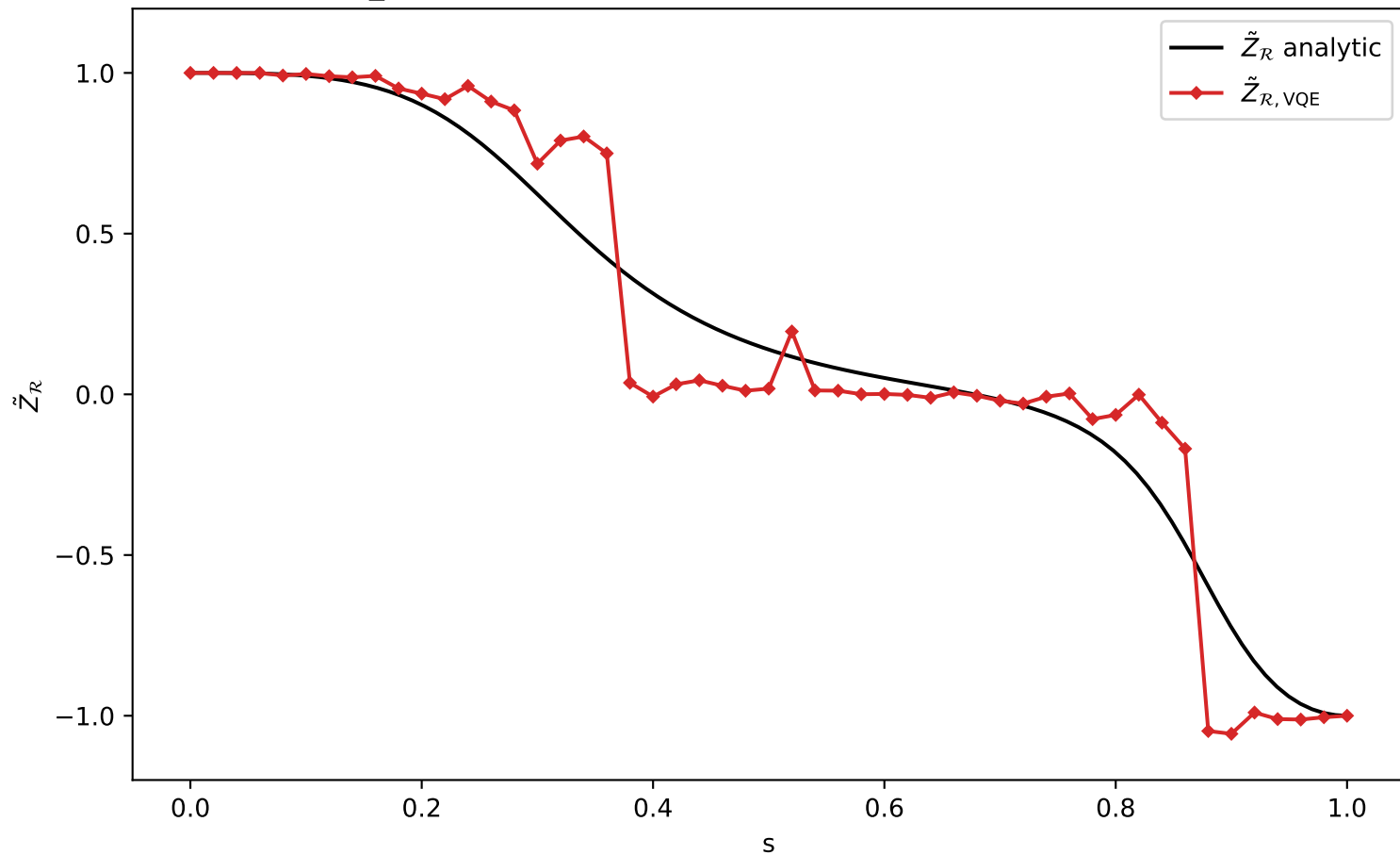
ZR_VQE-nosym vs analytic ZR, H (L=8, depth=5, delta=1)
