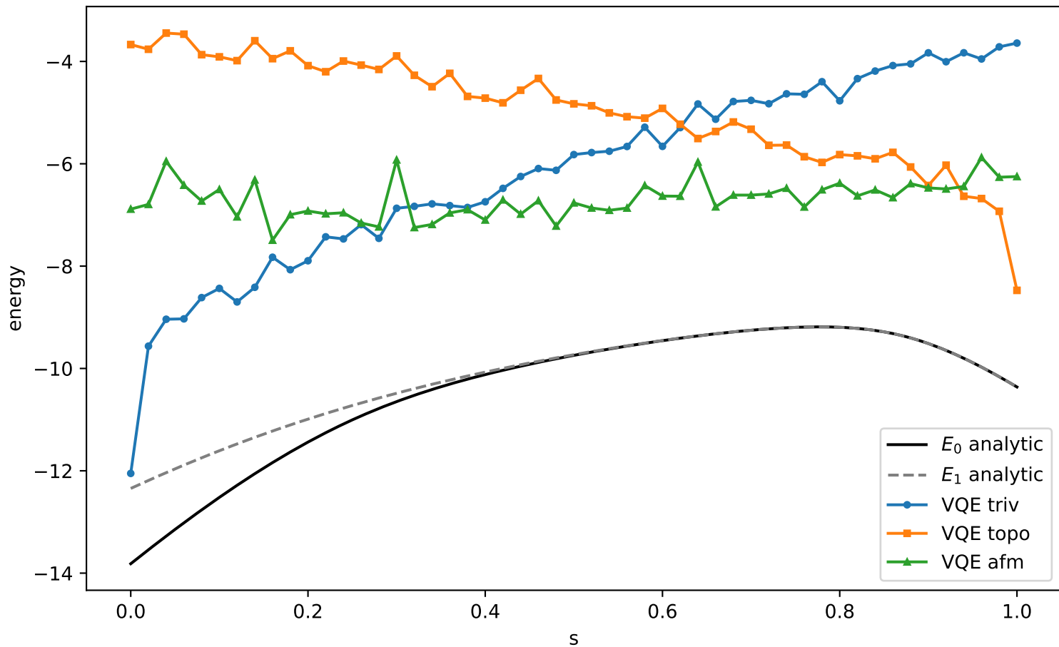
VQE hw sym depth1 delta=1.0 full
