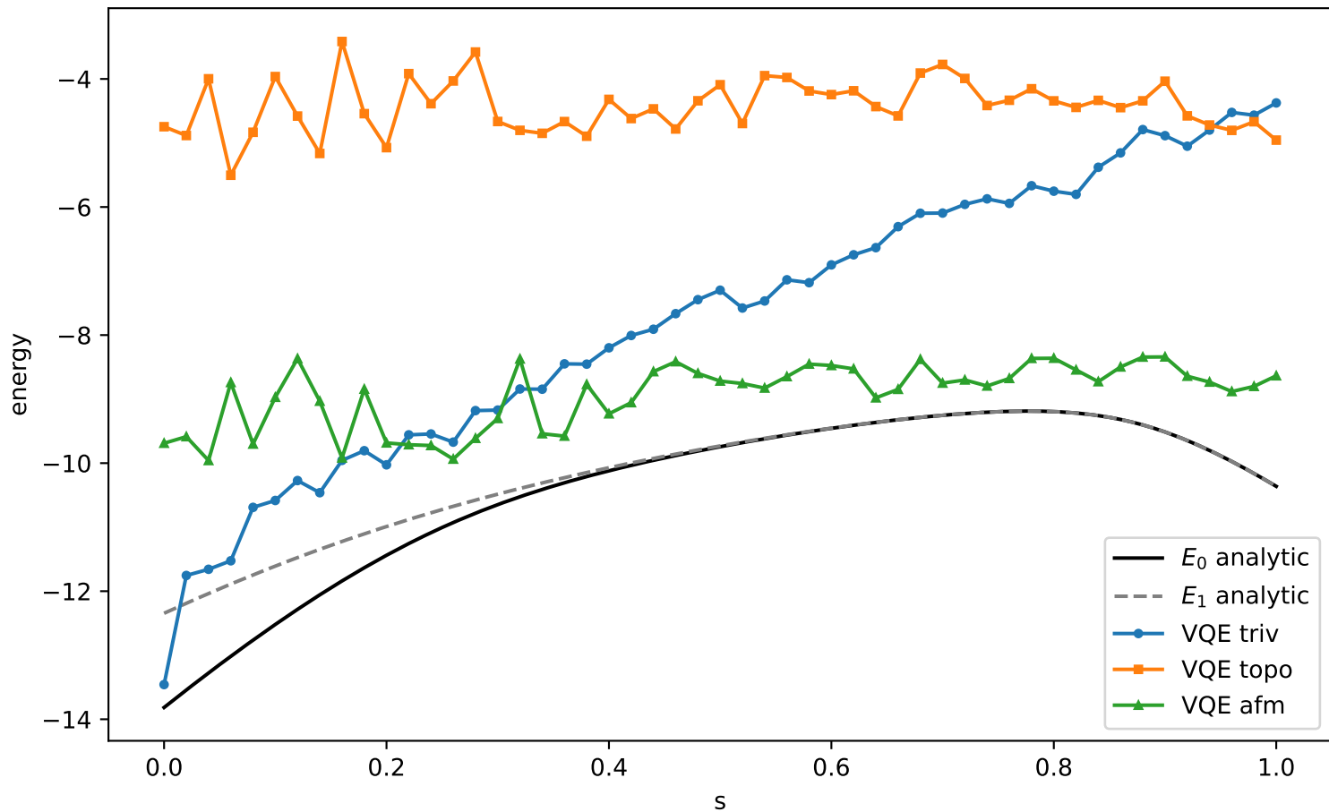
VQE postselect nosym depth1 delta=1.0 full-Hpost (diagnostic)
