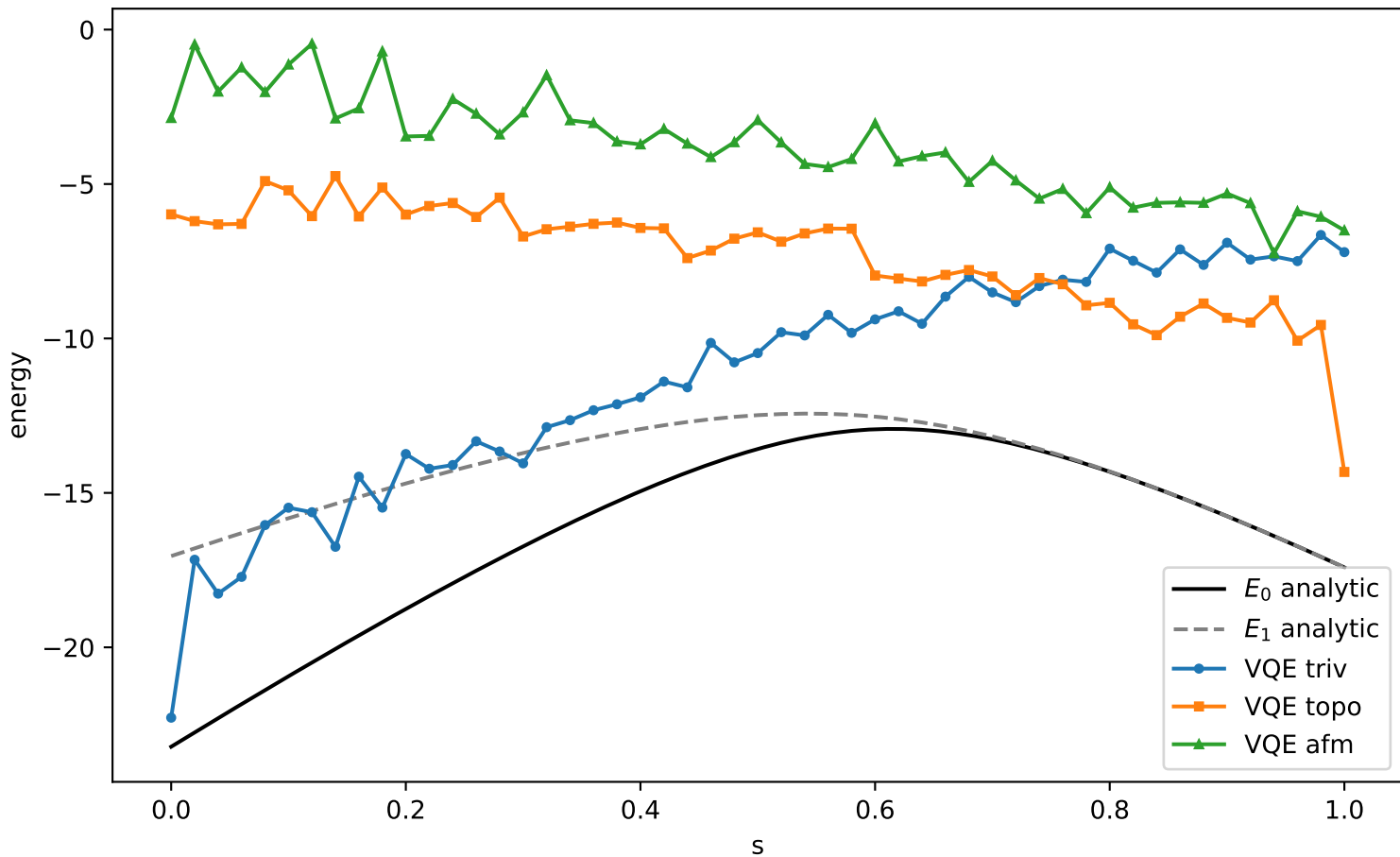
VQE postselect sym depth1 delta=-1.0 full-Hpost (diagnostic)
