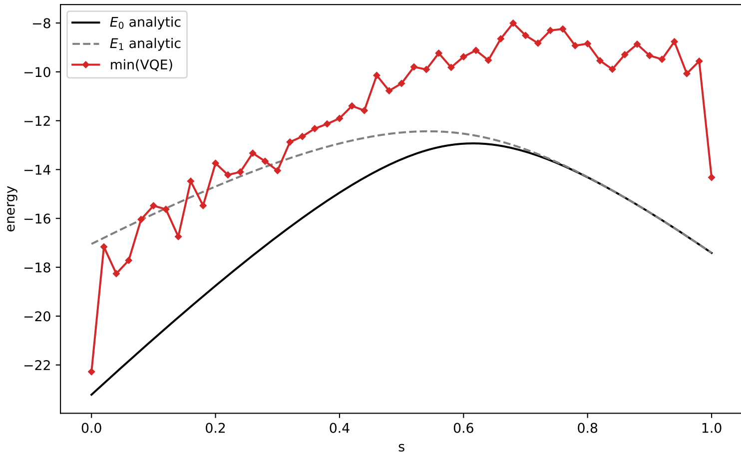
VQE postselect sym depth1 delta=-1.0 min-Hpost (diagnostic)
