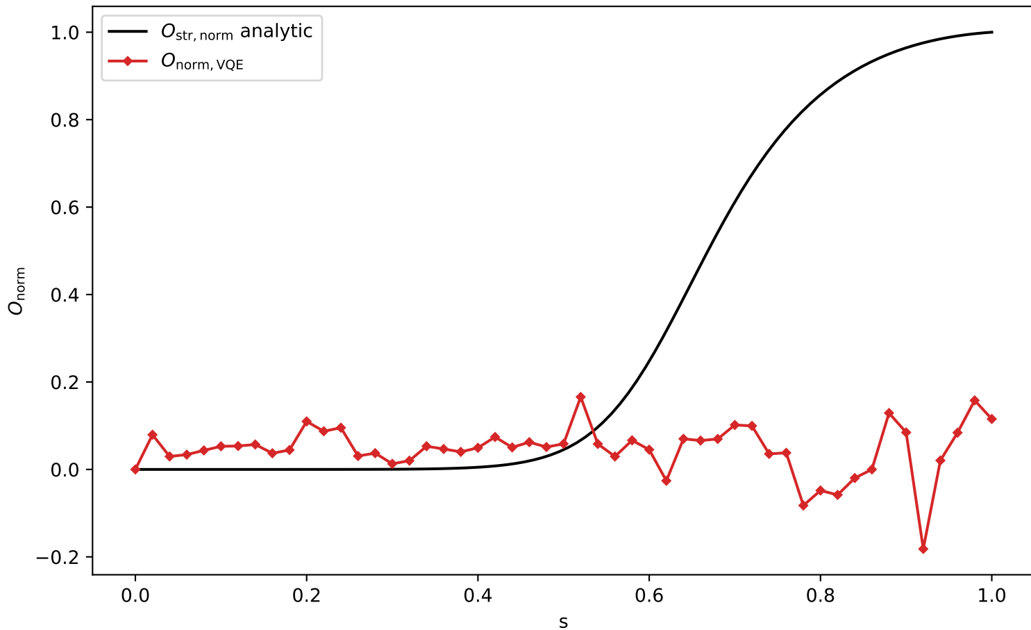
VQE postselect nosym depth1 delta=-1.0 o
