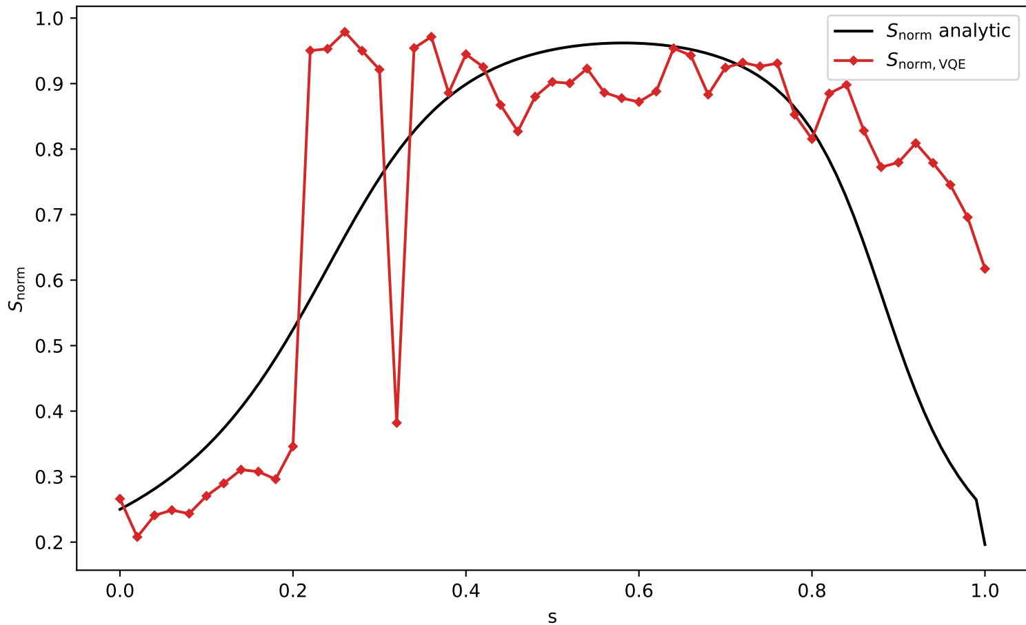
VQE postselect nosym depth1 delta=1.0 s
