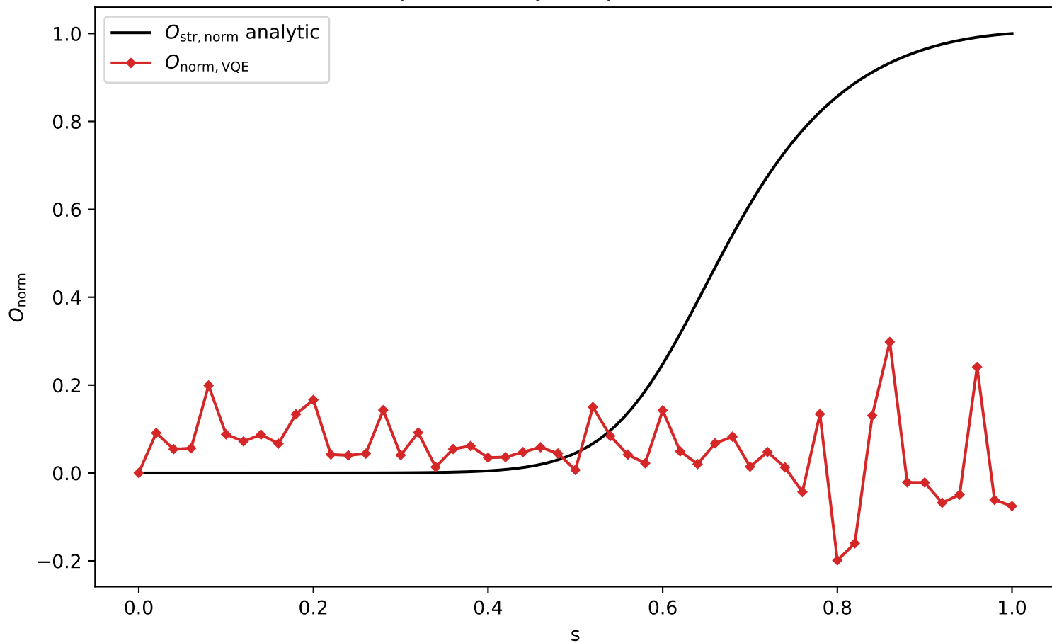
VQE postselect sym depth1 delta=-1.0 o
