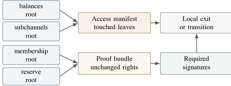
Figure 7: Factory proof mode. A local transition must expose the leaves it touches and prove that the relevant untouched rights are unchanged.
