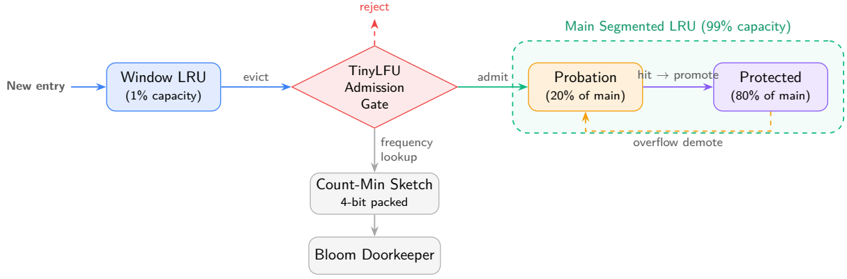
Figure 6: W-TinyLFU three-segment architecture. New entries enter the window cache. When the window overflows, its LRU victim becomes a candidate for the main cache. If the main cache is full, the candidate competes against the probation segment’s LRU victim via the TinyLFU admission filter.
