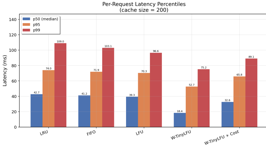
Figure 10: Per-request latency percentiles at cache size 200 (synthetic).
