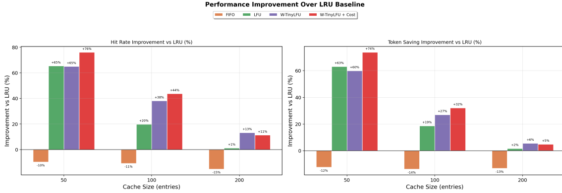
Figure 9: Percentage improvement over LRU baseline (synthetic).
