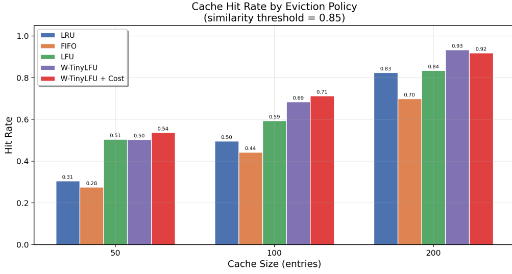
Figure 7: Hit rate by cache size on synthetic Zipfian workload (threshold = 0.85).
