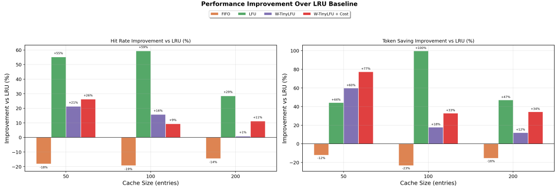
Figure 15: Improvement over LRU on LMSYS data (threshold = 0.85).
