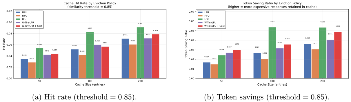
Figure 14: LMSYS results at stricter threshold (0.85). Hit rates drop \sim 40% vs. 0.80; W-TinyLFU+Cost leads token savings at cs = 50, while LFU leads at larger caches.
