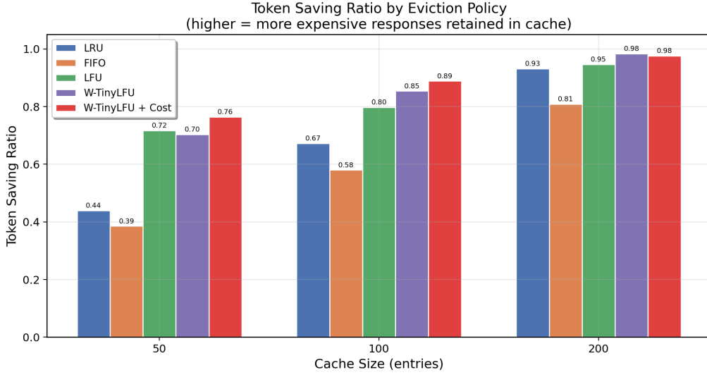
Figure 8: Token saving ratio by cache size (synthetic). The gap between hit rate and token savings confirms cost-aware caching of expensive responses.
