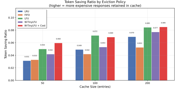
(b) Token saving ratio by cache size.
