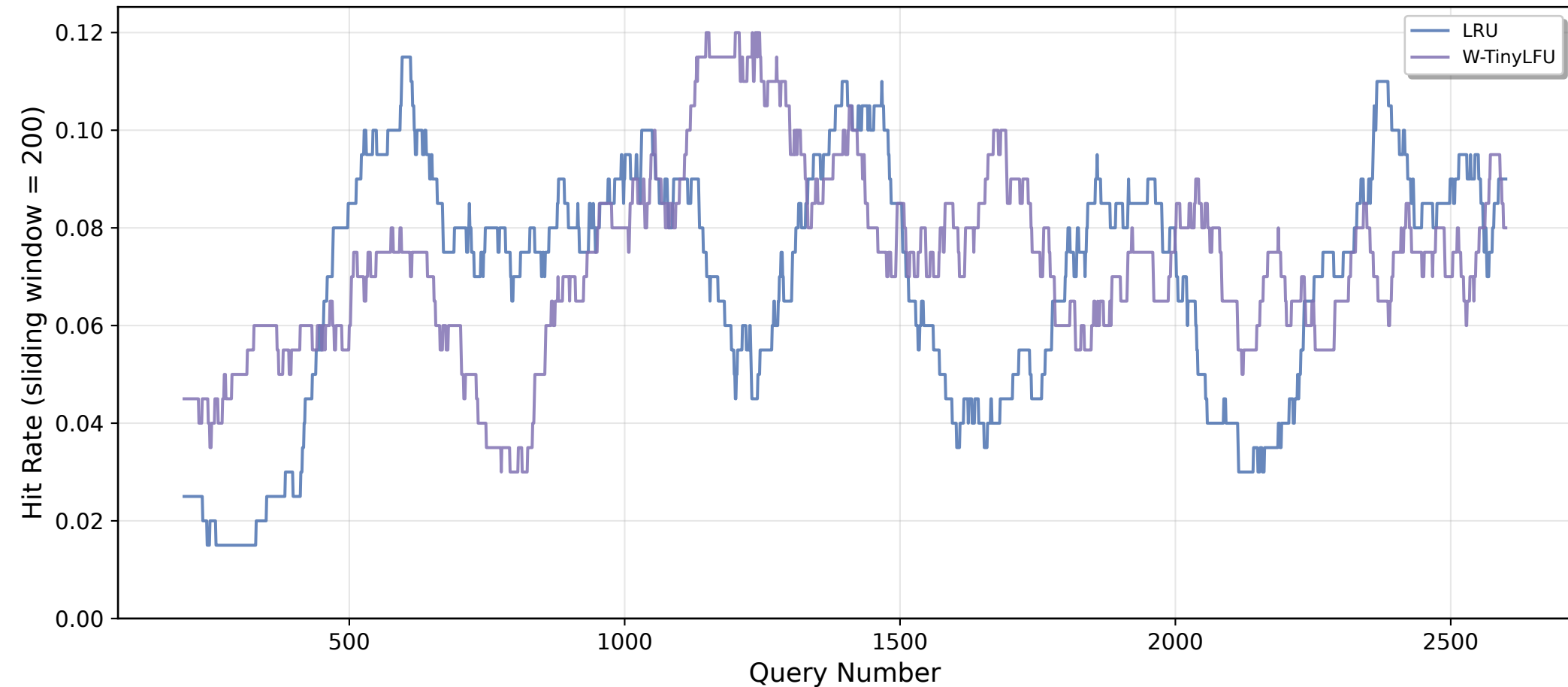
Cache Hit Rate Over Time (cache size = 200)
