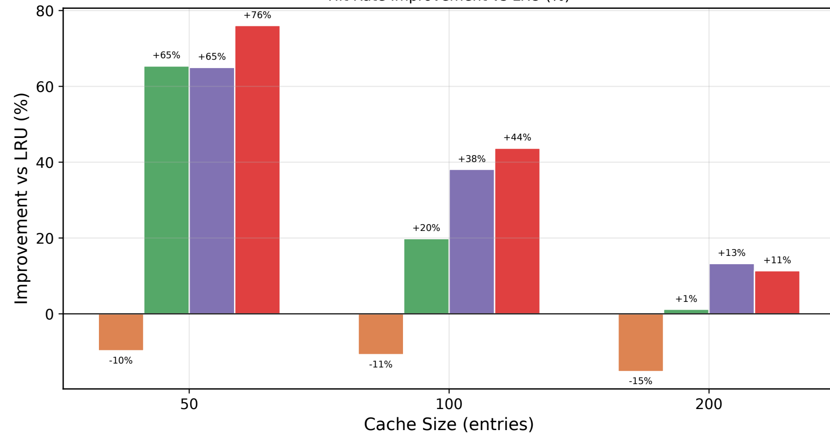
Hit Rate Improvement vs LRU (%)
