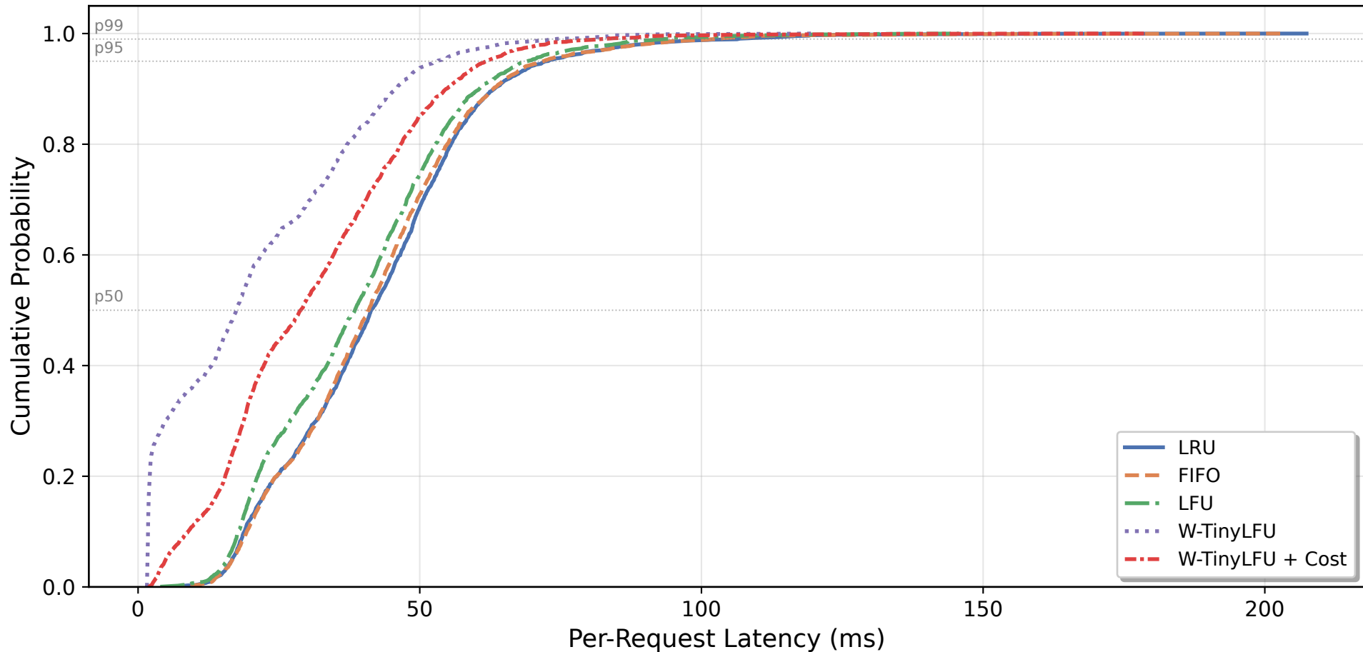
Latency CDF by Eviction Policy (cache size = 200)
