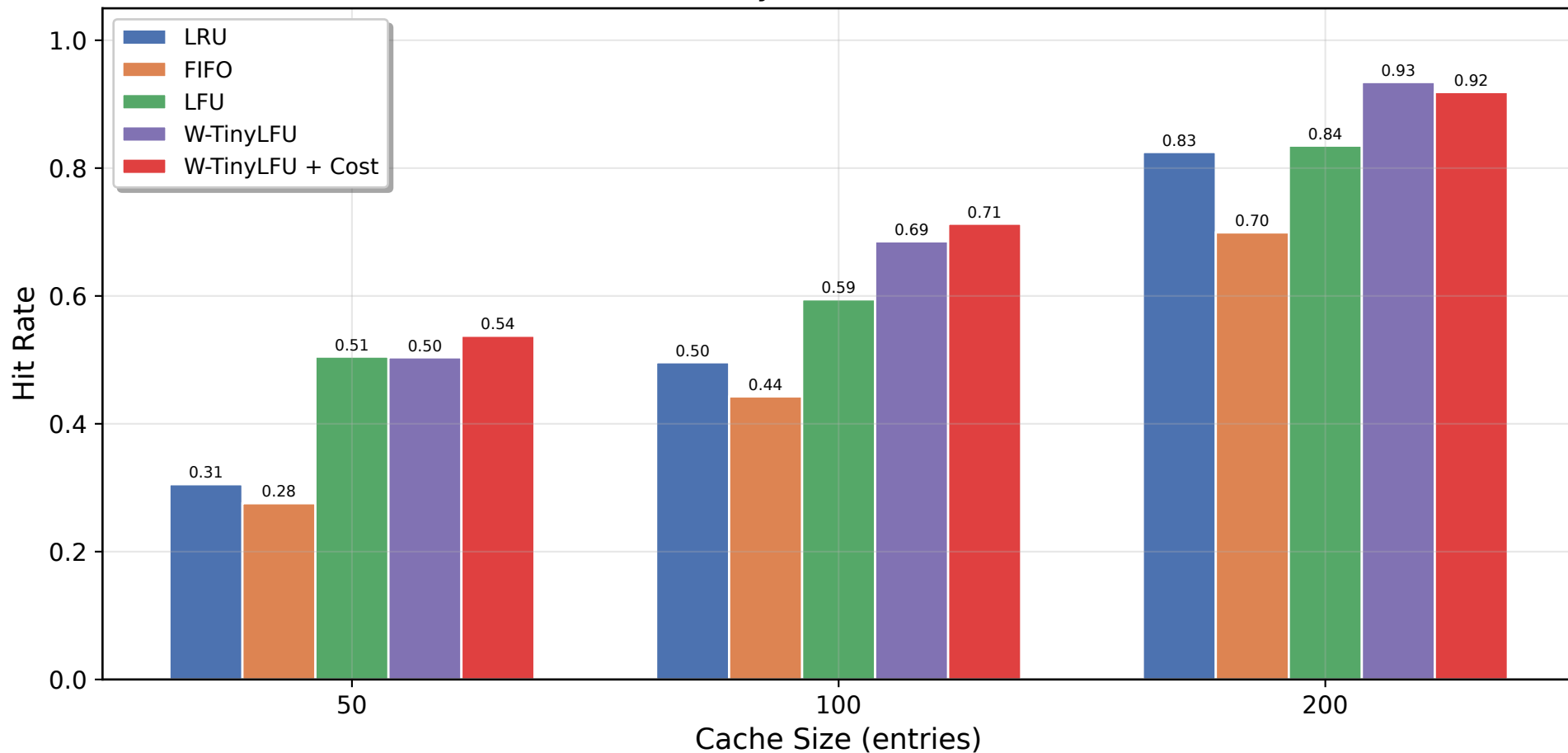
Cache Hit Rate by Eviction Policy (similarity threshold = 0.85)
